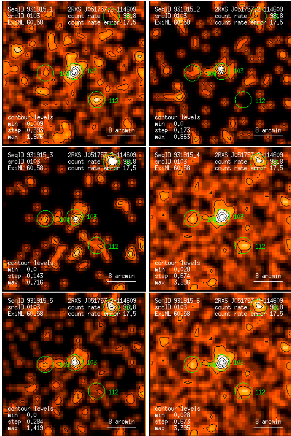
Figure 103: RASS 931915: detection 0103: band rate images, Gaussian filter: (1) PSPC channels 11 – 41, (2) 52 – 90, (3) 91 – 201, (4) 11 – 235, (5) 52 – 201, (6) 11 – 201. Broad band rates in counts/ks. Band rate contour levels in counts/ks/arcmin 2 .
