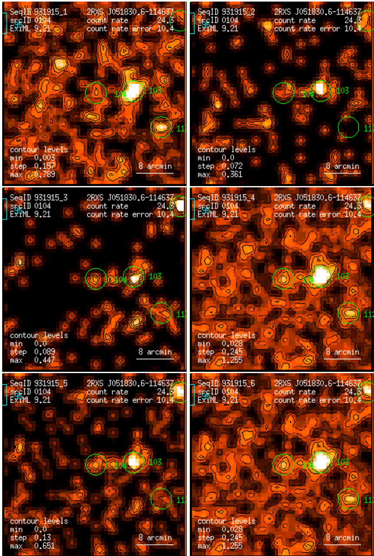
Figure 104: RASS 931915: detection 0104: band rate images, Gaussian filter: (1) PSPC channels 11 – 41, (2) 52 – 90, (3) 91 – 201, (4) 11 – 235, (5) 52 – 201, (6) 11 – 201. Broad band rates in counts/ks. Band rate contour levels in counts/ks/arcmin 2 .
