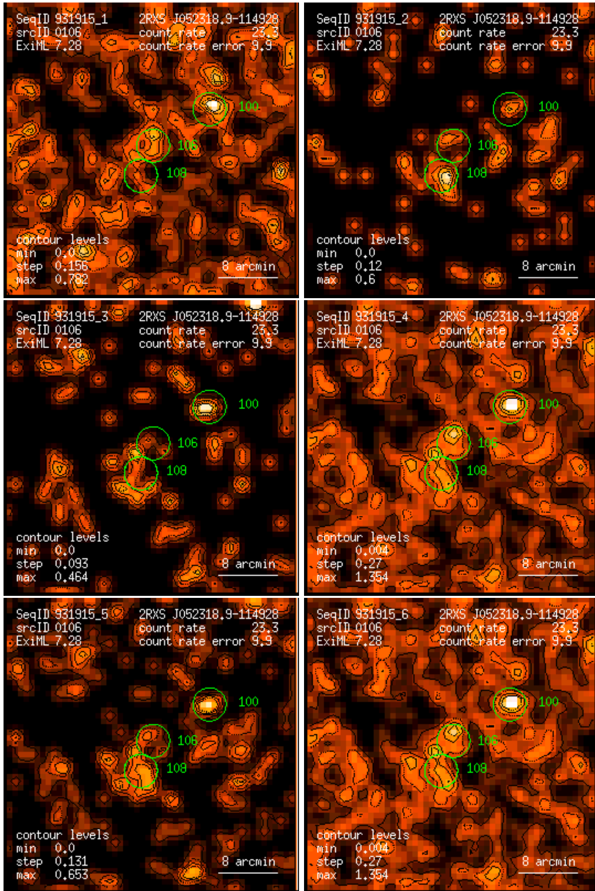
Figure 106: RASS 931915: detection 0106: band rate images, Gaussian filter: (1) PSPC channels 11 – 41, (2) 52 – 90, (3) 91 – 201, (4) 11 – 235, (5) 52 – 201, (6) 11 – 201. Broad band rates in counts/ks. Band rate contour levels in counts/ks/arcmin 2 .
