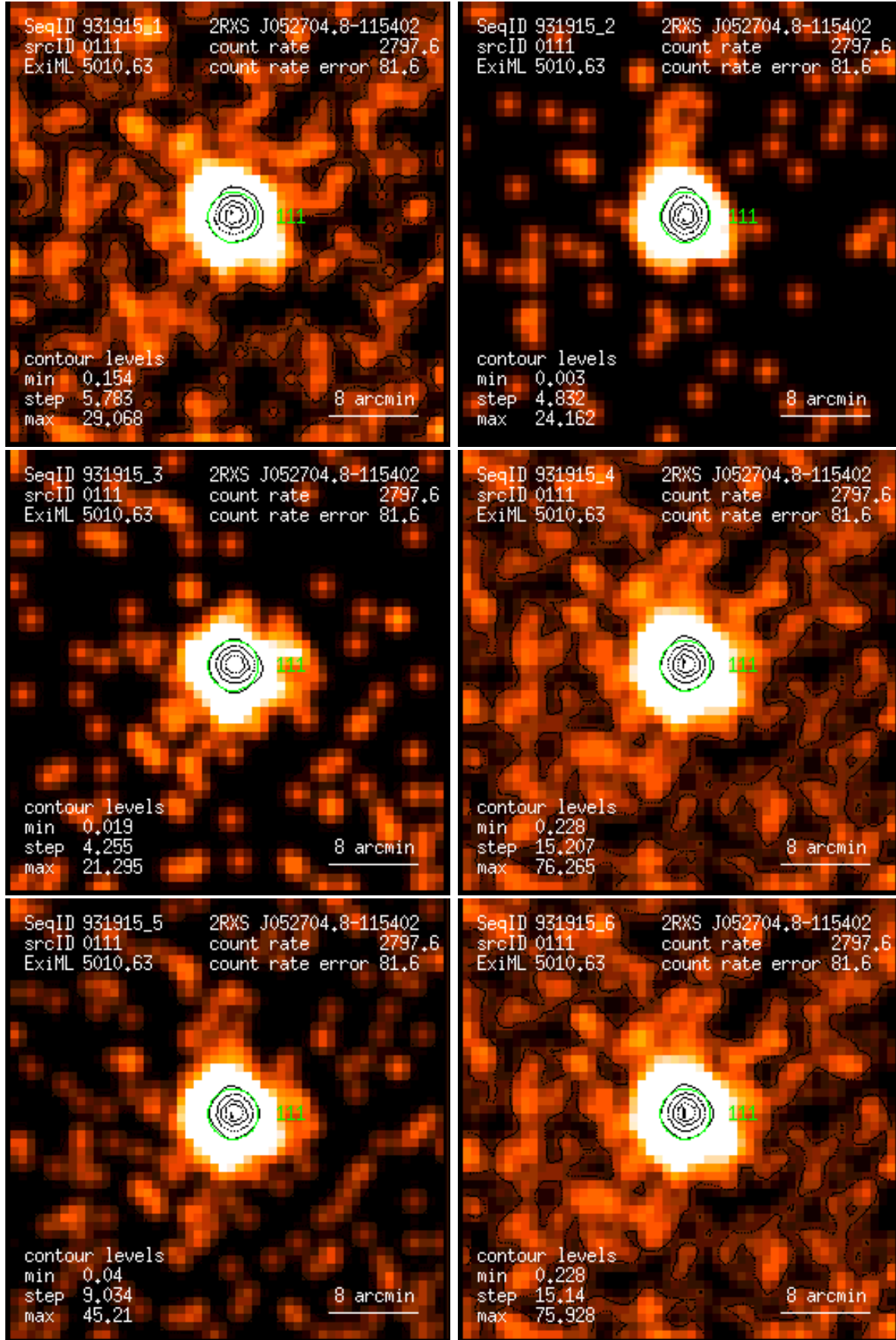
Figure 111: RASS 931915: detection 0111: band rate images, Gaussian filter: (1) PSPC channels 11 – 41, (2) 52 – 90, (3) 91 – 201, (4) 11 – 235, (5) 52 – 201, (6) 11 – 201. Broad band rates in counts/ks. Band rate contour levels in counts/ks/arcmin 2 .
