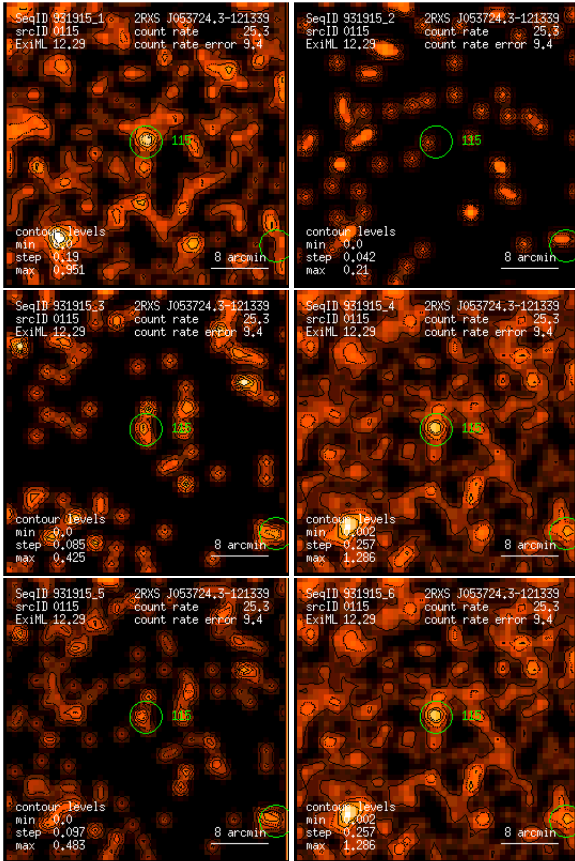
Figure 115: RASS 931915: detection 0115: band rate images, Gaussian filter: (1) PSPC channels 11 – 41, (2) 52 – 90, (3) 91 – 201, (4) 11 – 235, (5) 52 – 201, (6) 11 – 201. Broad band rates in counts/ks. Band rate contour levels in counts/ks/arcmin 2 .
