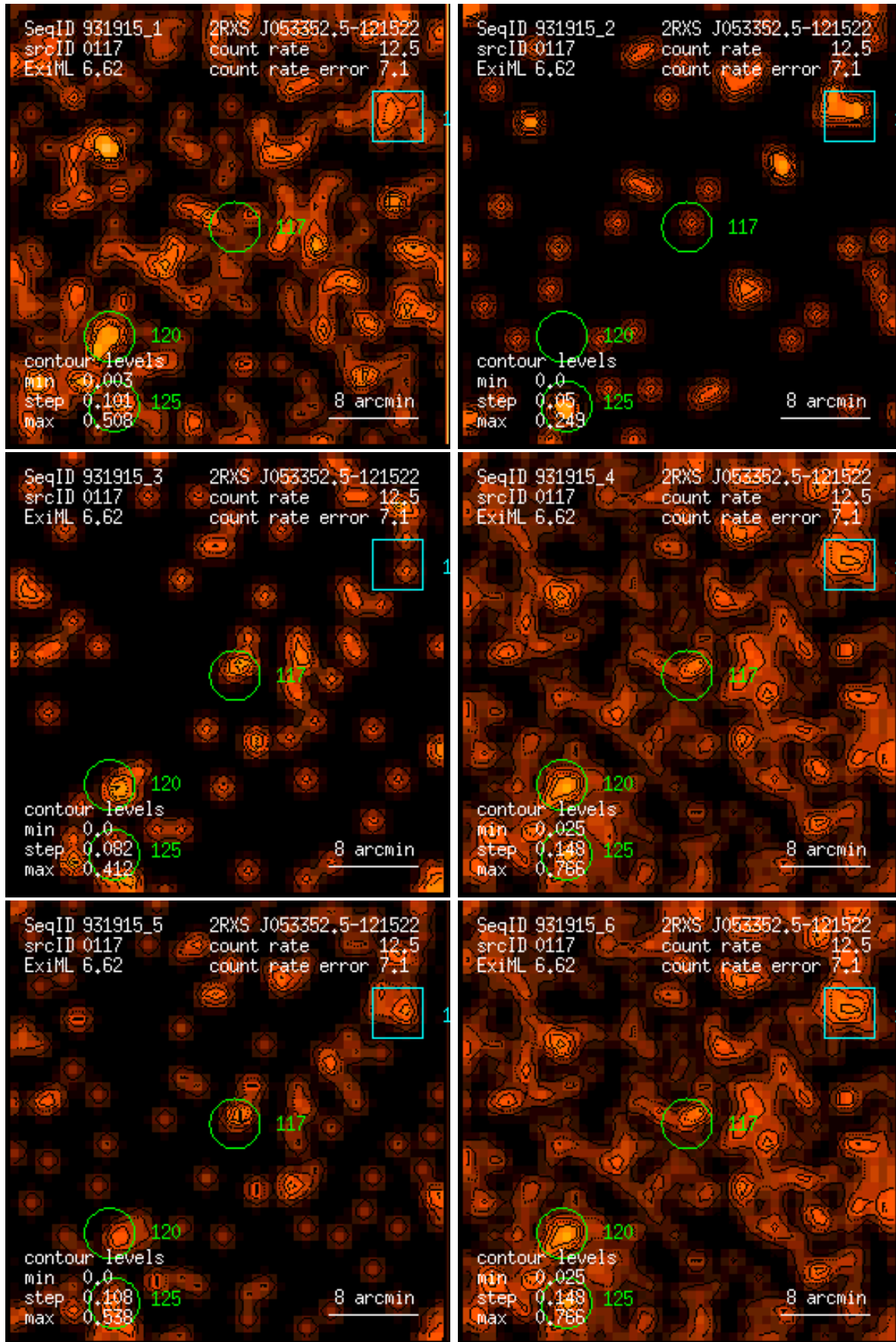
Figure 117: RASS 931915: detection 0117: band rate images, Gaussian filter: (1) PSPC channels 11 – 41, (2) 52 – 90, (3) 91 – 201, (4) 11 – 235, (5) 52 – 201, (6) 11 – 201. Broad band rates in counts/ks. Band rate contour levels in counts/ks/arcmin 2 .
