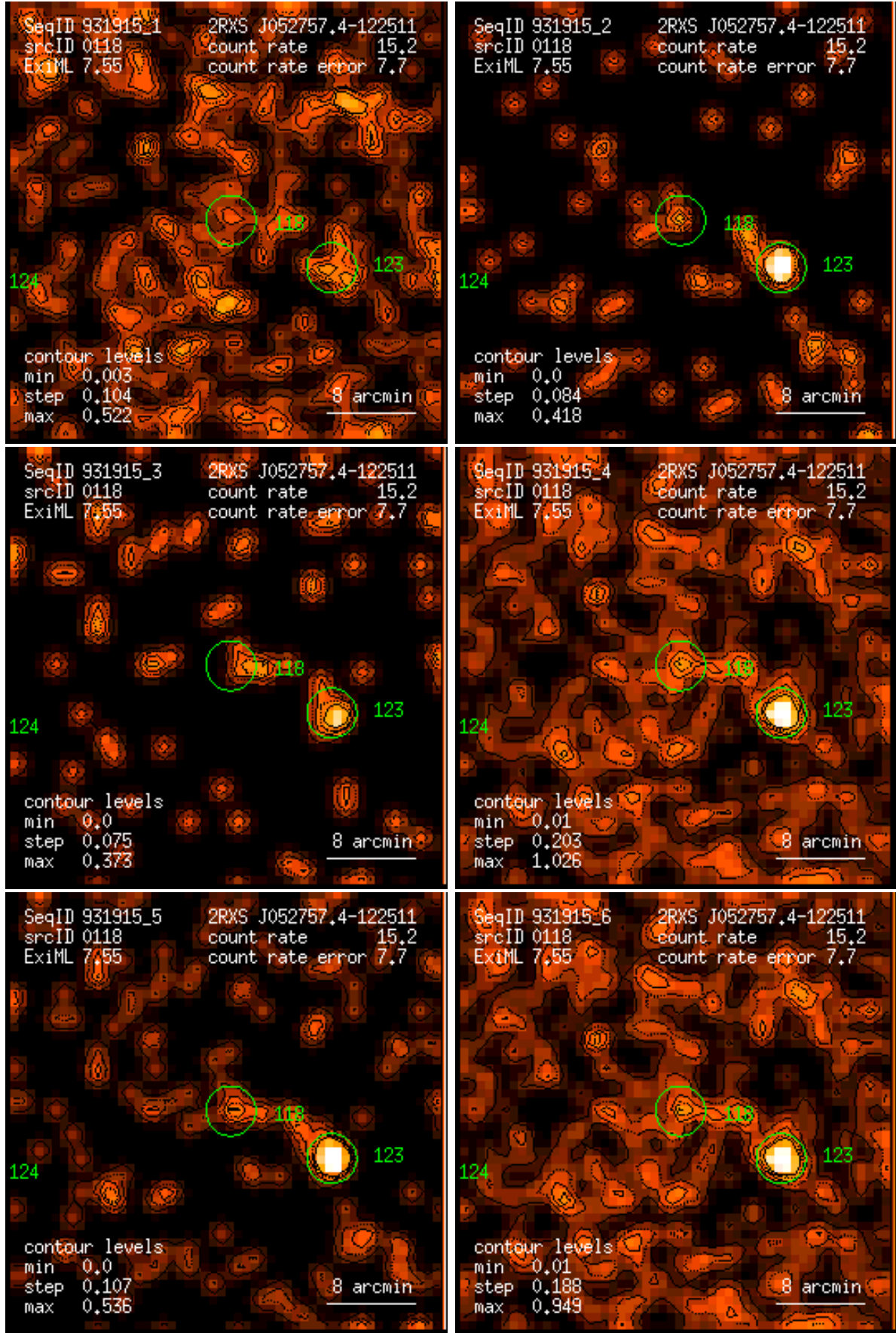
Figure 118: RASS 931915: detection 0118: band rate images, Gaussian filter: (1) PSPC channels 11 – 41, (2) 52 – 90, (3) 91 – 201, (4) 11 – 235, (5) 52 – 201, (6) 11 – 201. Broad band rates in counts/ks. Band rate contour levels in counts/ks/arcmin 2 .
