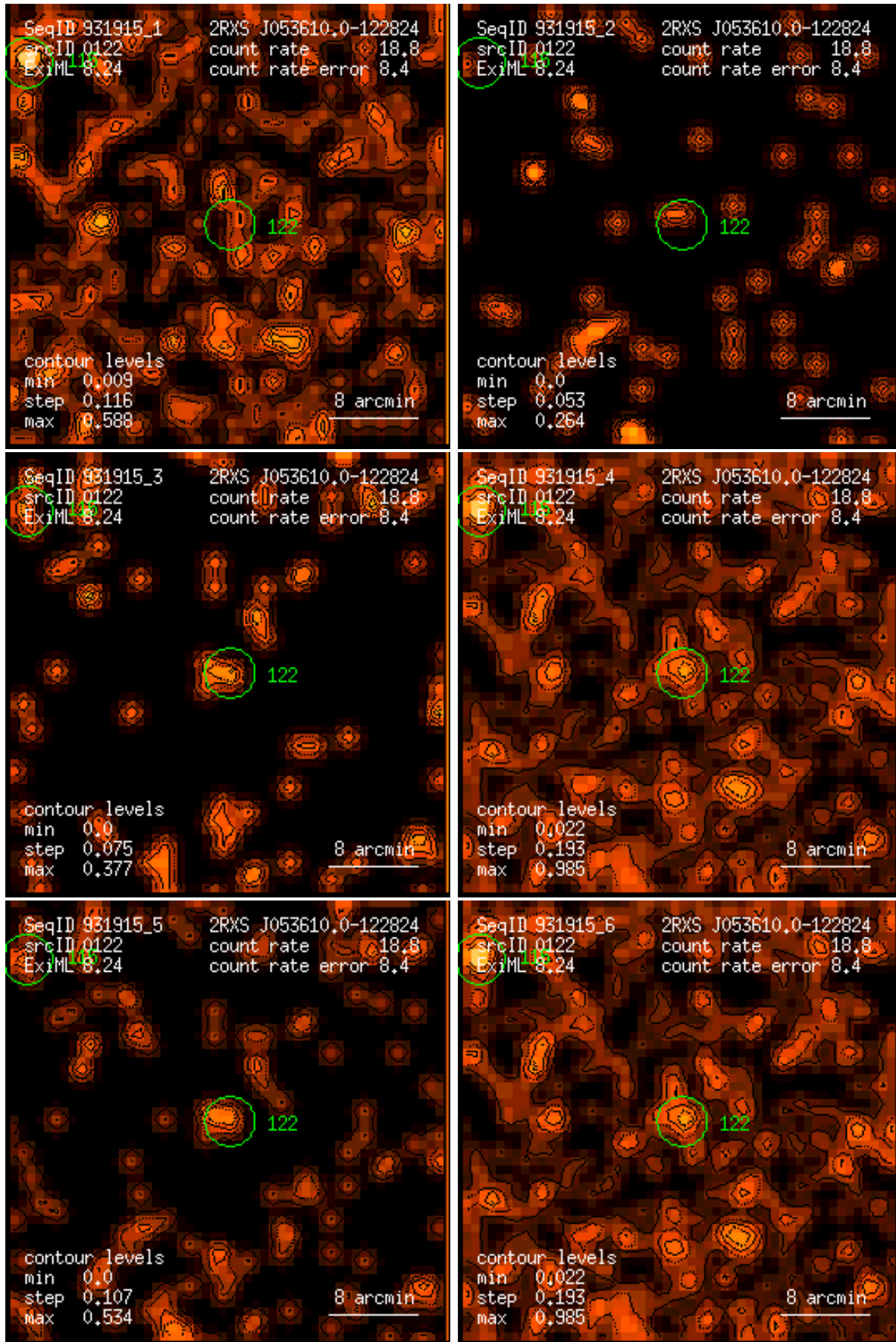
Figure 122: RASS 931915: detection 0122: band rate images, Gaussian filter: (1) PSPC channels 11 – 41, (2) 52 – 90, (3) 91 – 201, (4) 11 – 235, (5) 52 – 201, (6) 11 – 201. Broad band rates in counts/ks. Band rate contour levels in counts/ks/arcmin 2 .
