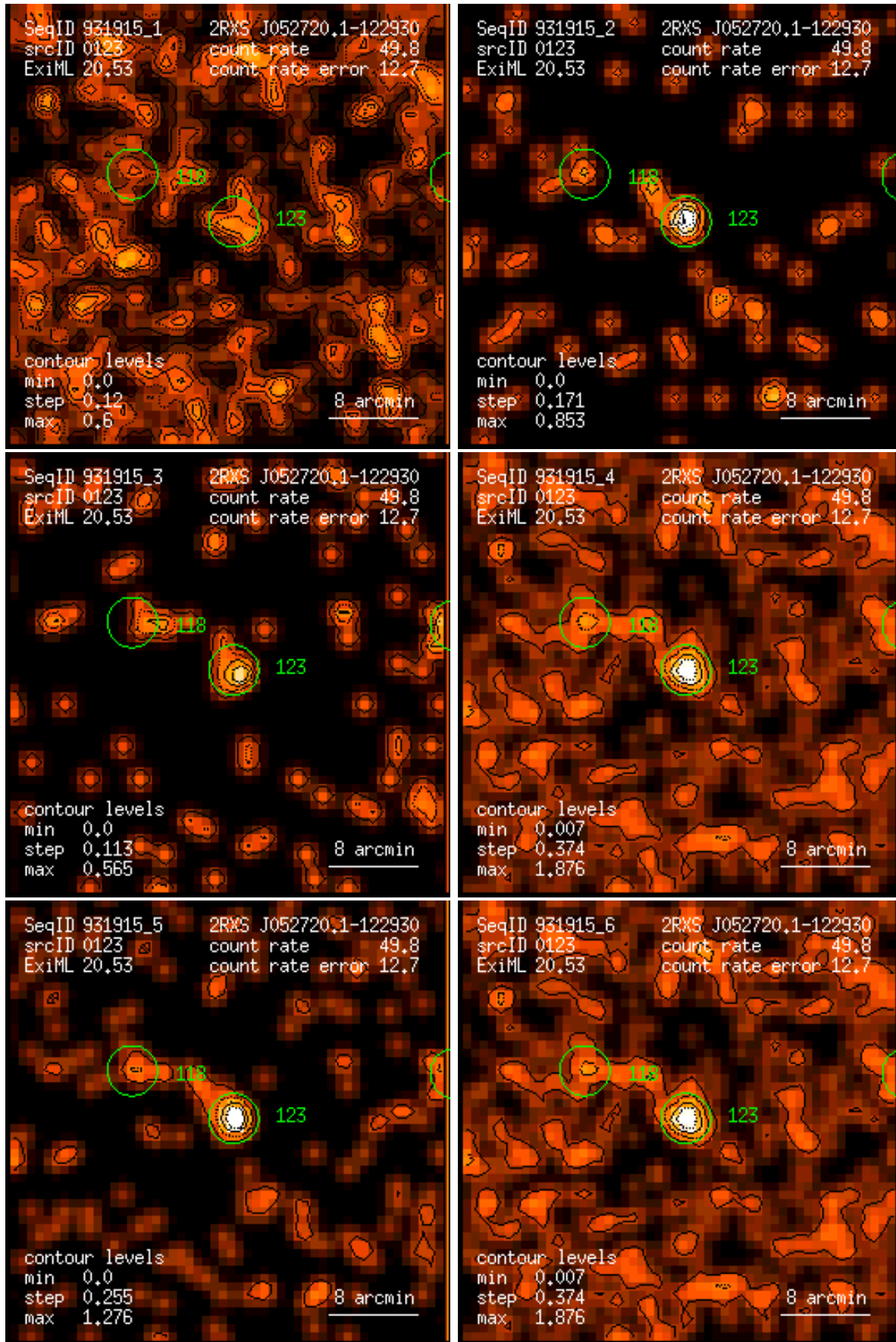
Figure 123: RASS 931915: detection 0123: band rate images, Gaussian filter: (1) PSPC channels 11 – 41, (2) 52 – 90, (3) 91 – 201, (4) 11 – 235, (5) 52 – 201, (6) 11 – 201. Broad band rates in counts/ks. Band rate contour levels in counts/ks/arcmin 2 .
