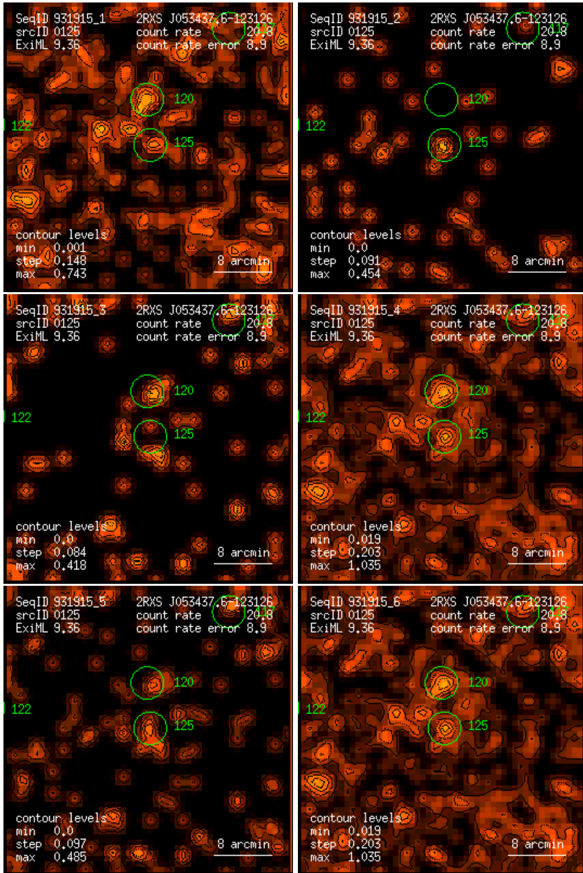
Figure 125: RASS 931915: detection 0125: band rate images, Gaussian filter: (1) PSPC channels 11 – 41, (2) 52 – 90, (3) 91 – 201, (4) 11 – 235, (5) 52 – 201, (6) 11 – 201. Broad band rates in counts/ks. Band rate contour levels in counts/ks/arcmin 2 .
