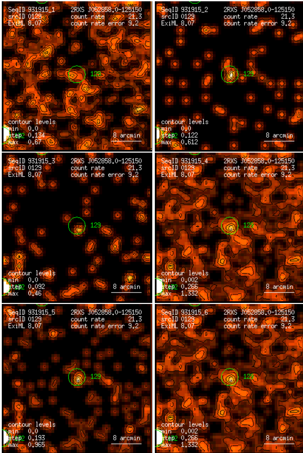
Figure 129: RASS 931915: detection 0129: band rate images, Gaussian filter: (1) PSPC channels 11 – 41, (2) 52 – 90, (3) 91 – 201, (4) 11 – 235, (5) 52 – 201, (6) 11 – 201. Broad band rates in counts/ks. Band rate contour levels in counts/ks/arcmin 2 .
