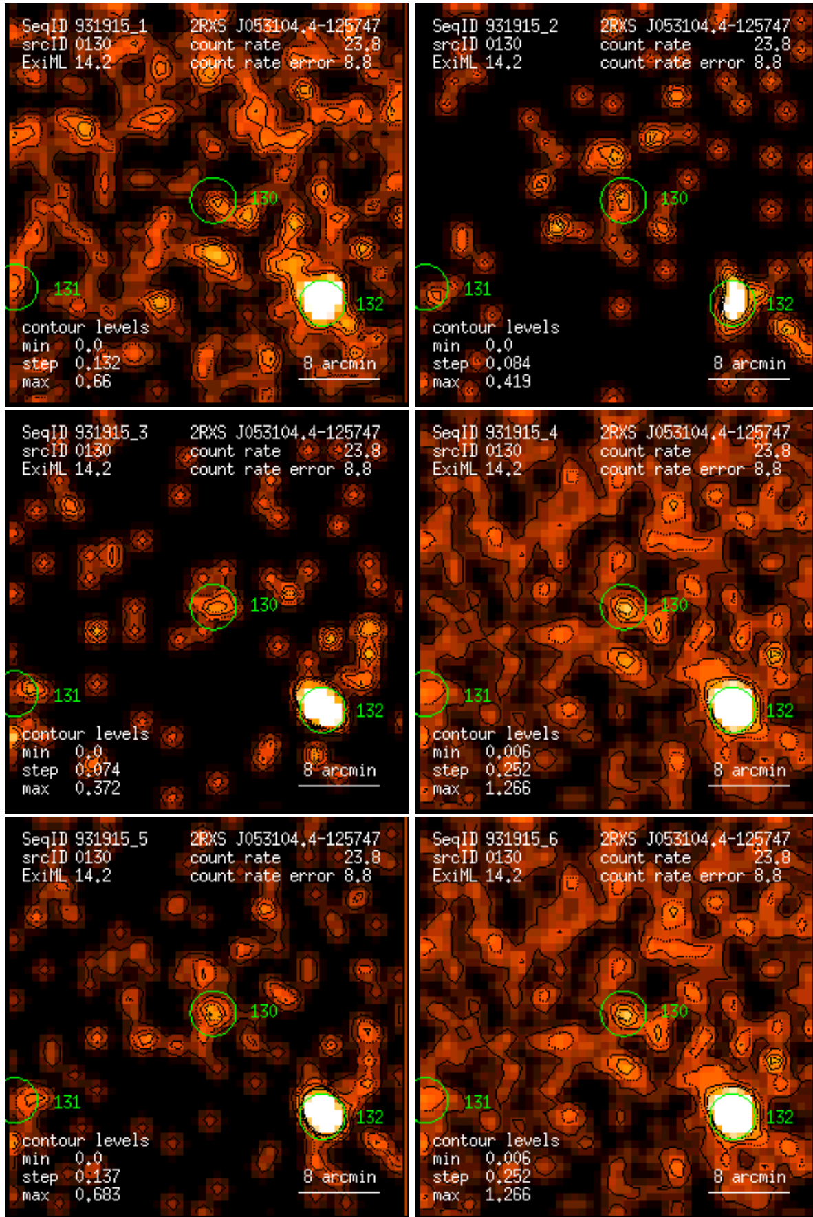
Figure 130: RASS 931915: detection 0130: band rate images, Gaussian filter: (1) PSPC channels 11 – 41, (2) 52 – 90, (3) 91 – 201, (4) 11 – 235, (5) 52 – 201, (6) 11 – 201. Broad band rates in counts/ks. Band rate contour levels in counts/ks/arcmin 2 .
