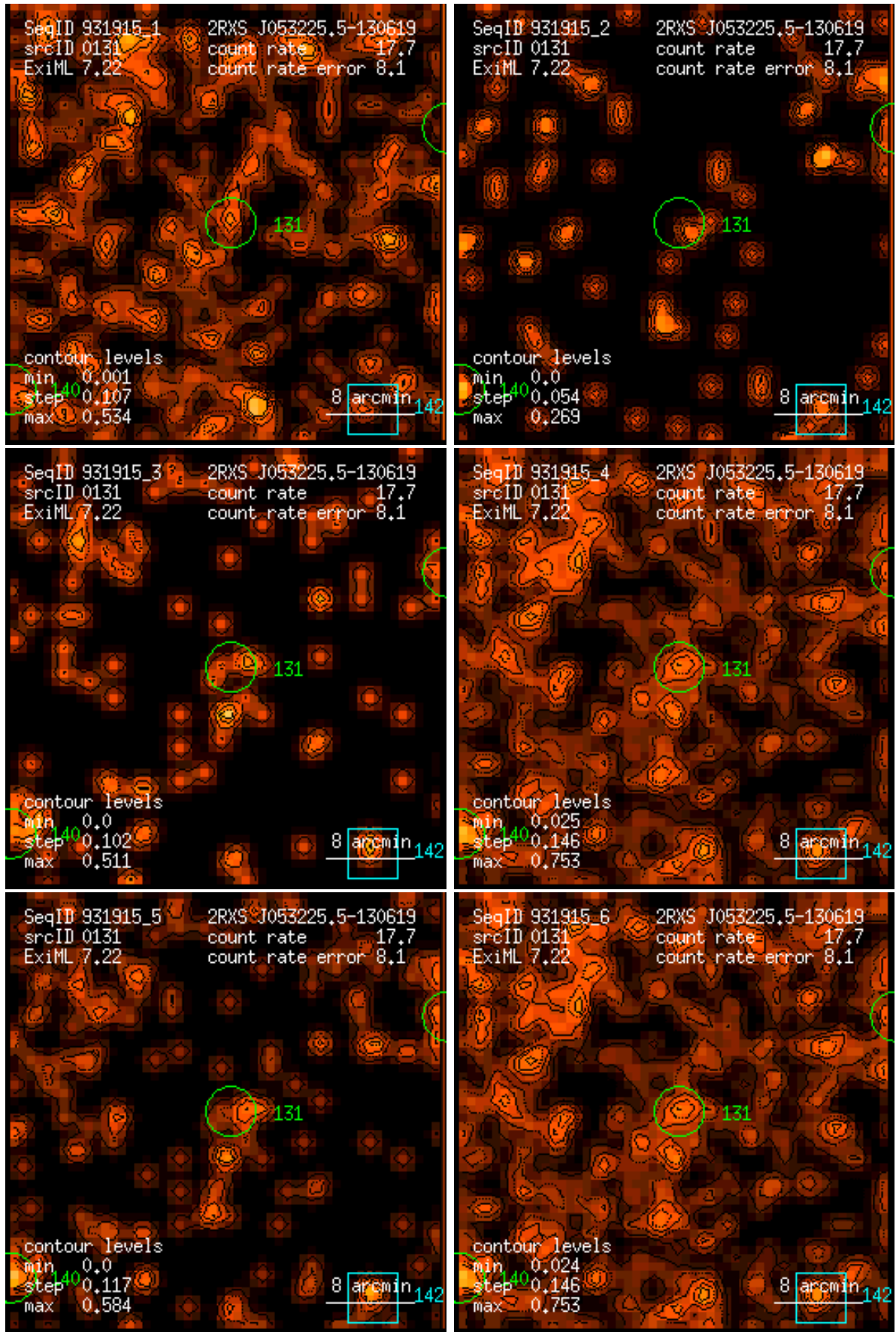
Figure 131: RASS 931915: detection 0131: band rate images, Gaussian filter: (1) PSPC channels 11 – 41, (2) 52 – 90, (3) 91 – 201, (4) 11 – 235, (5) 52 – 201, (6) 11 – 201. Broad band rates in counts/ks. Band rate contour levels in counts/ks/arcmin 2 .
