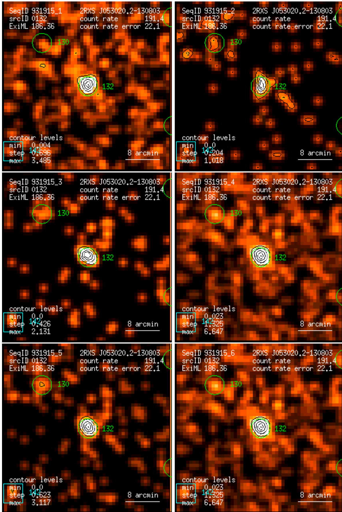
Figure 132: RASS 931915: detection 0132: band rate images, Gaussian filter: (1) PSPC channels 11 – 41, (2) 52 – 90, (3) 91 – 201, (4) 11 – 235, (5) 52 – 201, (6) 11 – 201. Broad band rates in counts/ks. Band rate contour levels in counts/ks/arcmin 2 .
