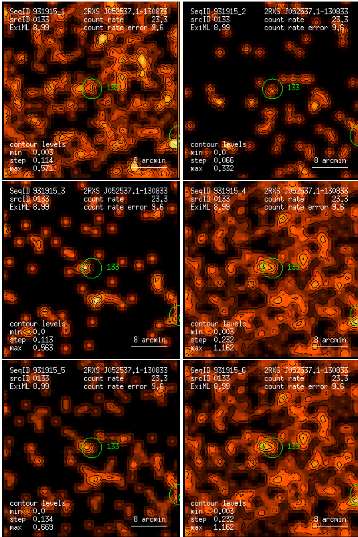
Figure 133: RASS 931915: detection 0133: band rate images, Gaussian filter: (1) PSPC channels 11 – 41, (2) 52 – 90, (3) 91 – 201, (4) 11 – 235, (5) 52 – 201, (6) 11 – 201. Broad band rates in counts/ks. Band rate contour levels in counts/ks/arcmin 2 .
