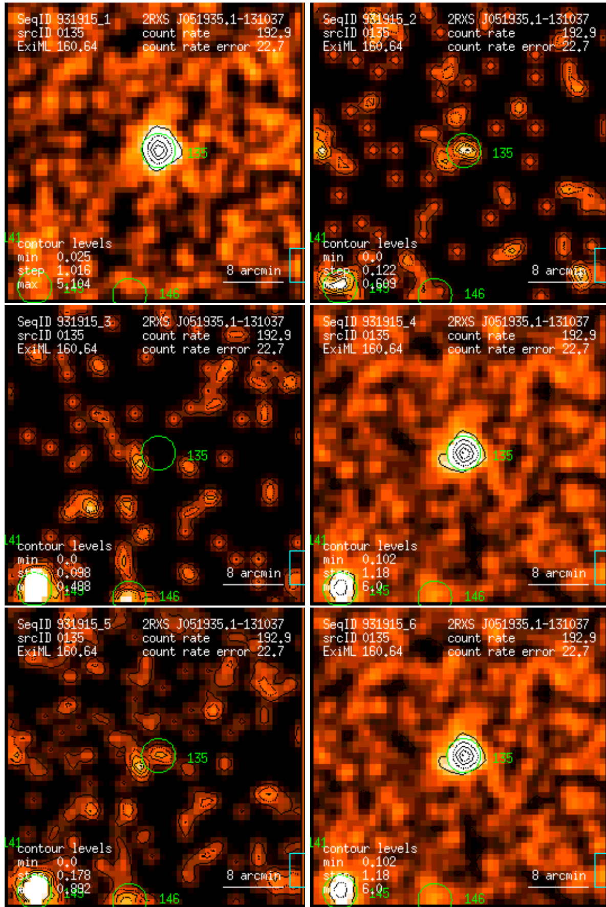
Figure 135: RASS 931915: detection 0135: band rate images, Gaussian filter: (1) PSPC channels 11 – 41, (2) 52 – 90, (3) 91 – 201, (4) 11 – 235, (5) 52 – 201, (6) 11 – 201. Broad band rates in counts/ks. Band rate contour levels in counts/ks/arcmin 2 .
