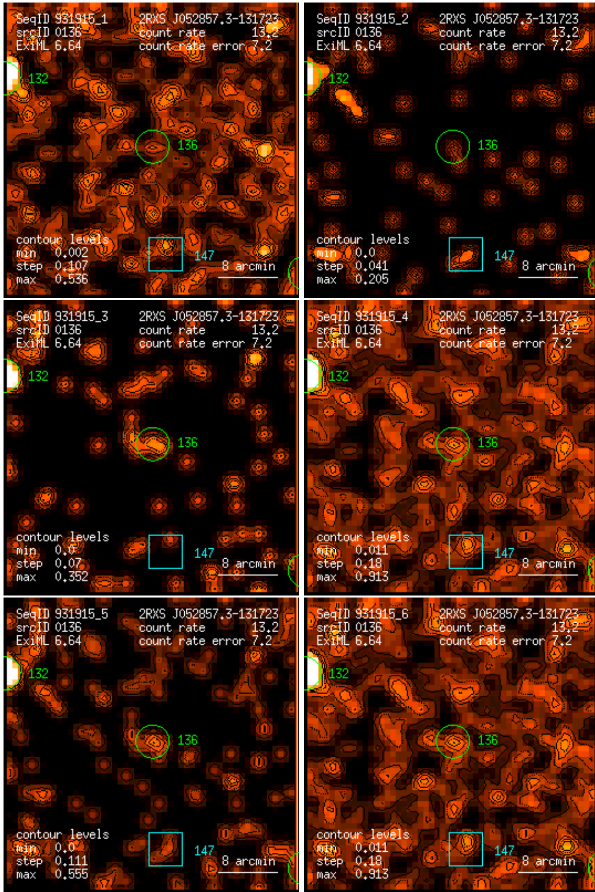
Figure 136: RASS 931915: detection 0136: band rate images, Gaussian filter: (1) PSPC channels 11 – 41, (2) 52 – 90, (3) 91 – 201, (4) 11 – 235, (5) 52 – 201, (6) 11 – 201. Broad band rates in counts/ks. Band rate contour levels in counts/ks/arcmin 2 .
