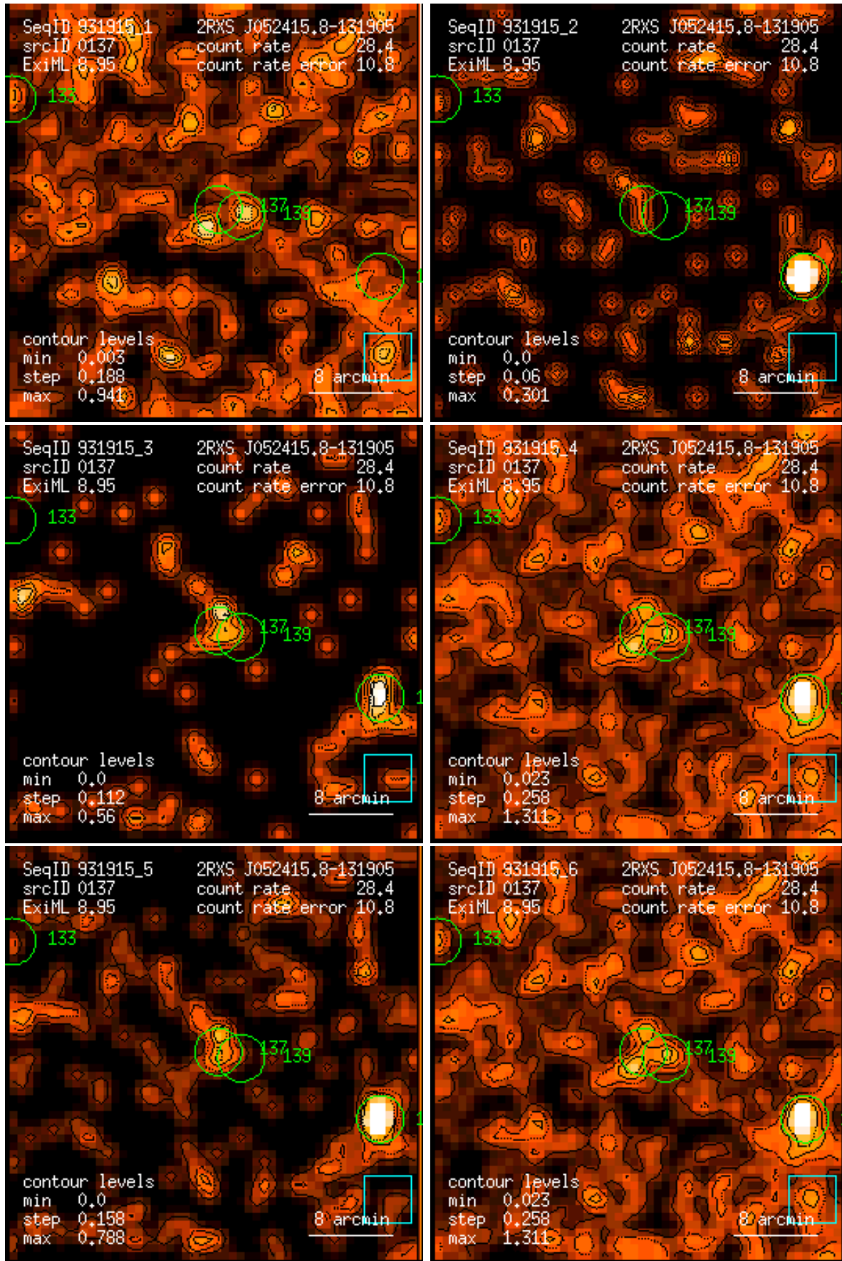
Figure 137: RASS 931915: detection 0137: band rate images, Gaussian filter: (1) PSPC channels 11 – 41, (2) 52 – 90, (3) 91 – 201, (4) 11 – 235, (5) 52 – 201, (6) 11 – 201. Broad band rates in counts/ks. Band rate contour levels in counts/ks/arcmin 2 .
