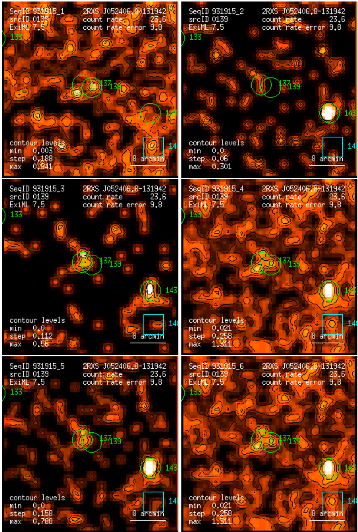
Figure 139: RASS 931915: detection 0139: band rate images, Gaussian filter: (1) PSPC channels 11 – 41, (2) 52 – 90, (3) 91 – 201, (4) 11 – 235, (5) 52 – 201, (6) 11 – 201. Broad band rates in counts/ks. Band rate contour levels in counts/ks/arcmin 2 .
