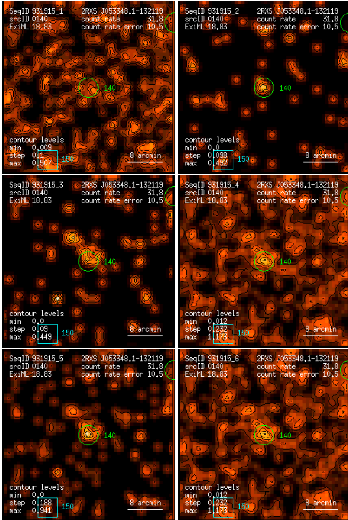
Figure 140: RASS 931915: detection 0140: band rate images, Gaussian filter: (1) PSPC channels 11 – 41, (2) 52 – 90, (3) 91 – 201, (4) 11 – 235, (5) 52 – 201, (6) 11 – 201. Broad band rates in counts/ks. Band rate contour levels in counts/ks/arcmin 2 .
