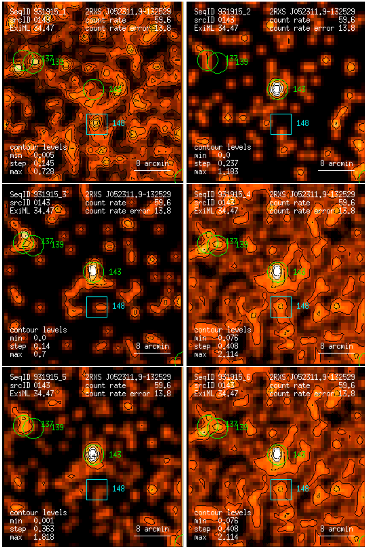
Figure 143: RASS 931915: detection 0143: band rate images, Gaussian filter: (1) PSPC channels 11 – 41, (2) 52 – 90, (3) 91 – 201, (4) 11 – 235, (5) 52 – 201, (6) 11 – 201. Broad band rates in counts/ks. Band rate contour levels in counts/ks/arcmin 2 .
