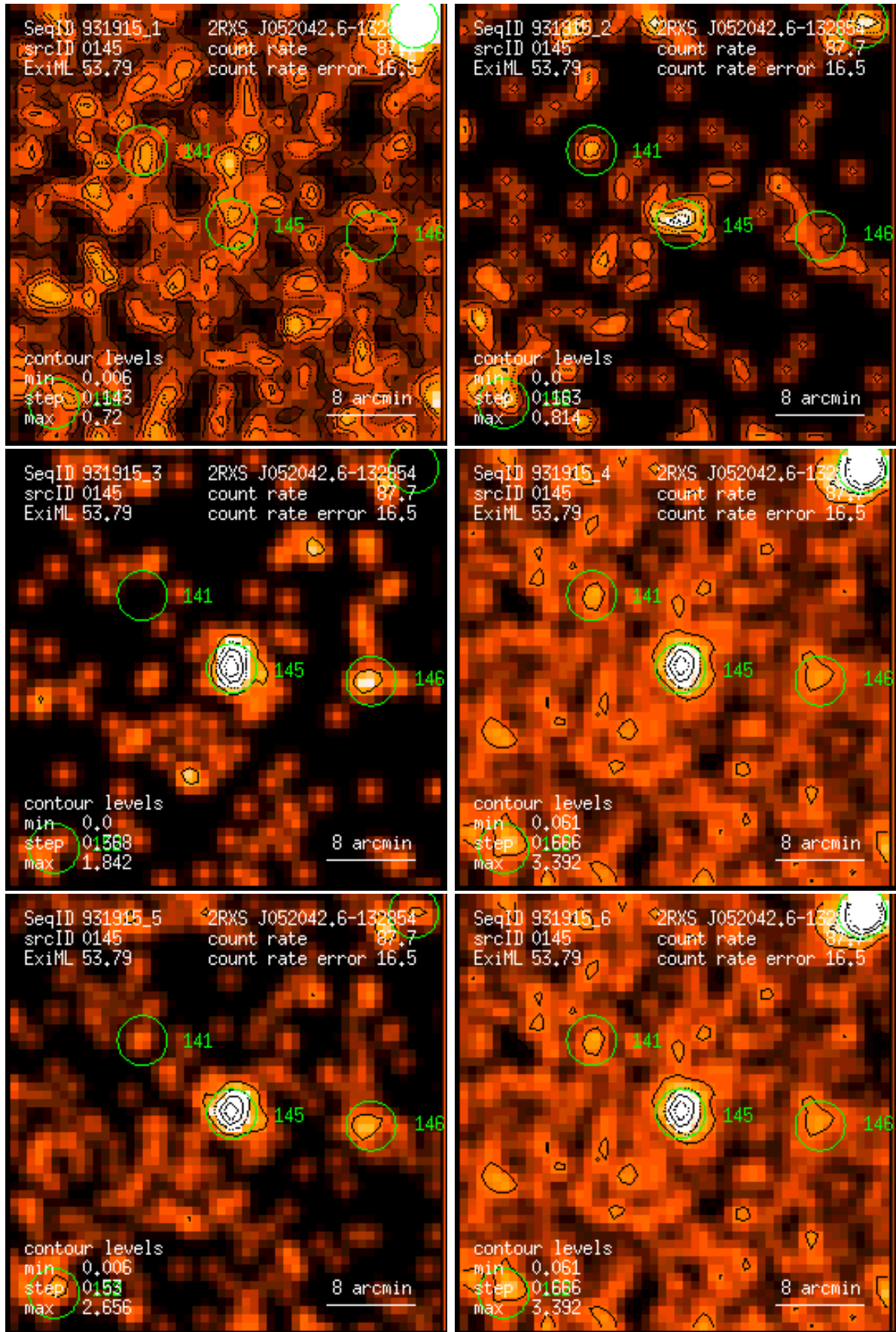
Figure 145: RASS 931915: detection 0145: band rate images, Gaussian filter: (1) PSPC channels 11 – 41, (2) 52 – 90, (3) 91 – 201, (4) 11 – 235, (5) 52 – 201, (6) 11 – 201. Broad band rates in counts/ks. Band rate contour levels in counts/ks/arcmin 2 .
