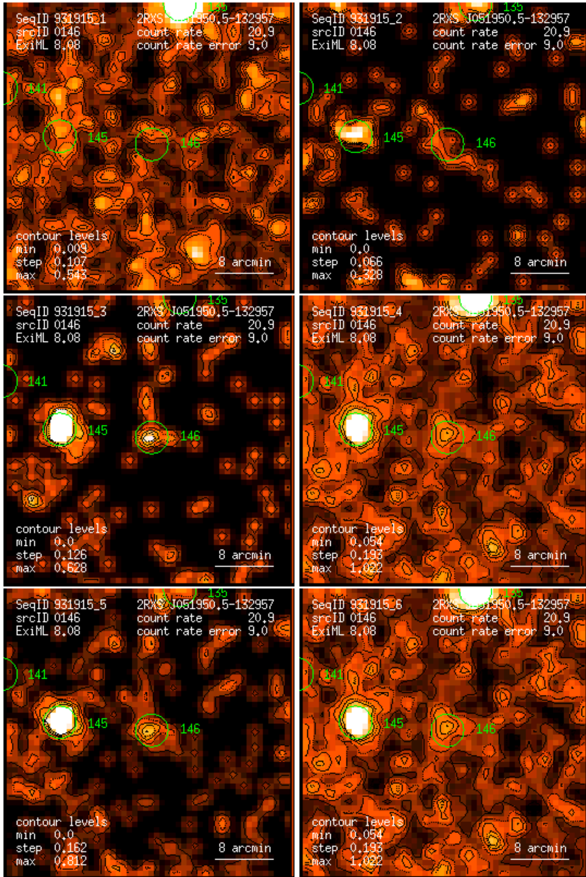
Figure 146: RASS 931915: detection 0146: band rate images, Gaussian filter: (1) PSPC channels 11 – 41, (2) 52 – 90, (3) 91 – 201, (4) 11 – 235, (5) 52 – 201, (6) 11 – 201. Broad band rates in counts/ks. Band rate contour levels in counts/ks/arcmin 2 .
