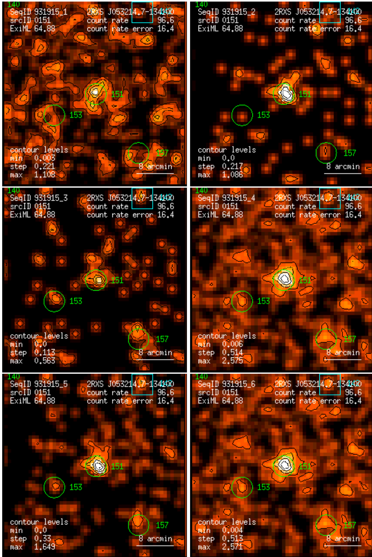
Figure 151: RASS 931915: detection 0151: band rate images, Gaussian filter: (1) PSPC channels 11 – 41, (2) 52 – 90, (3) 91 – 201, (4) 11 – 235, (5) 52 – 201, (6) 11 – 201. Broad band rates in counts/ks. Band rate contour levels in counts/ks/arcmin 2 .
