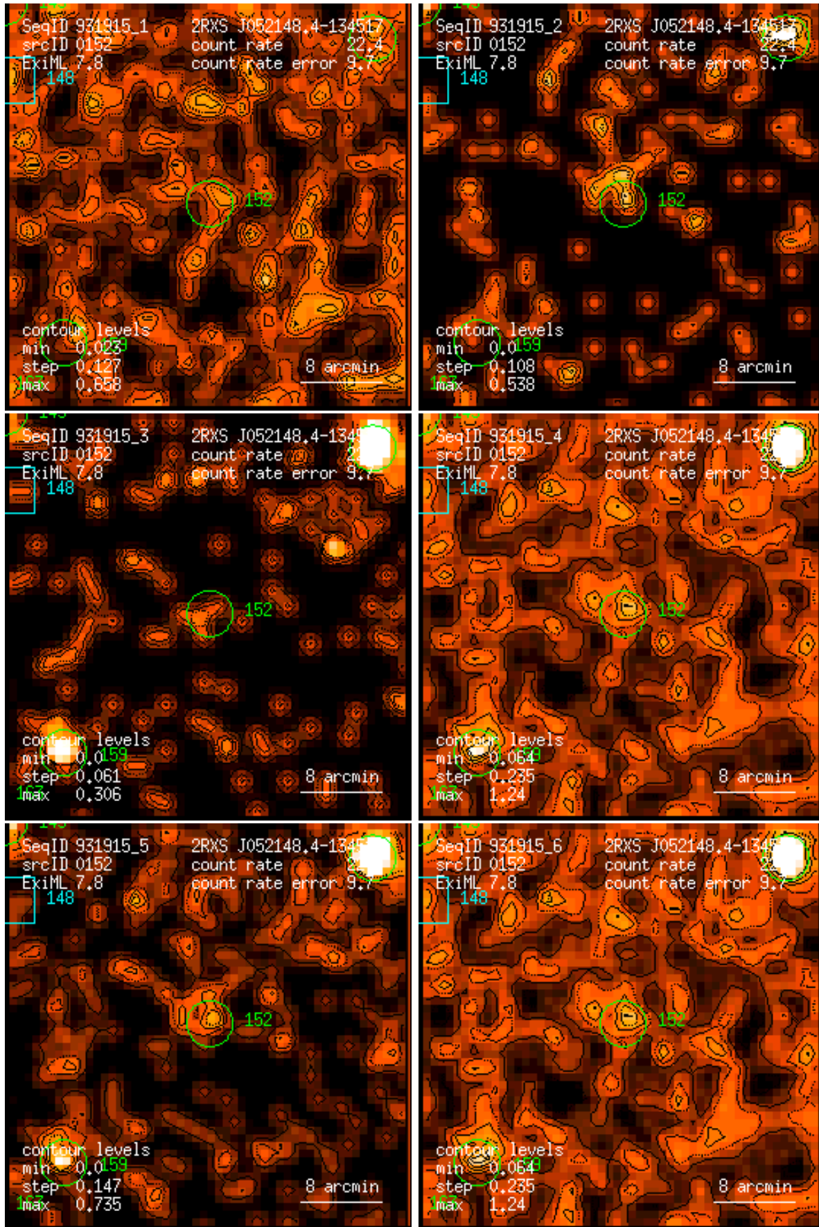
Figure 152: RASS 931915: detection 0152: band rate images, Gaussian filter: (1) PSPC channels 11 – 41, (2) 52 – 90, (3) 91 – 201, (4) 11 – 235, (5) 52 – 201, (6) 11 – 201. Broad band rates in counts/ks. Band rate contour levels in counts/ks/arcmin 2 .
