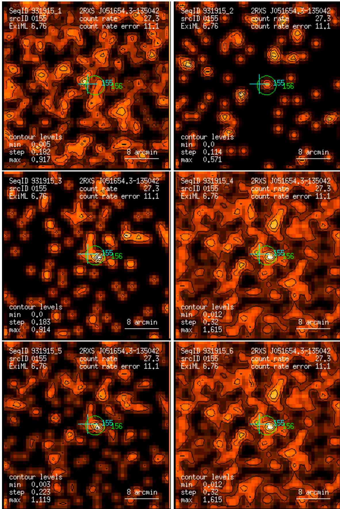
Figure 155: RASS 931915: detection 0155: band rate images, Gaussian filter: (1) PSPC channels 11 – 41, (2) 52 – 90, (3) 91 – 201, (4) 11 – 235, (5) 52 – 201, (6) 11 – 201. Broad band rates in counts/ks. Band rate contour levels in counts/ks/arcmin 2 .
