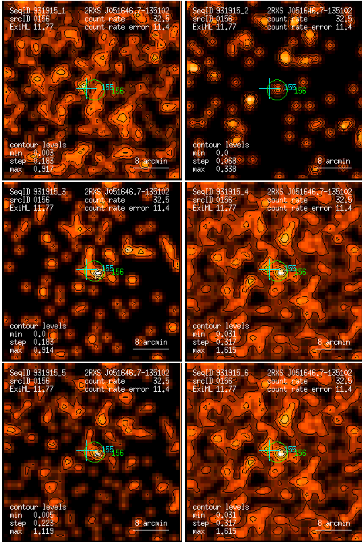
Figure 156: RASS 931915: detection 0156: band rate images, Gaussian filter: (1) PSPC channels 11 – 41, (2) 52 – 90, (3) 91 – 201, (4) 11 – 235, (5) 52 – 201, (6) 11 – 201. Broad band rates in counts/ks. Band rate contour levels in counts/ks/arcmin 2 .
