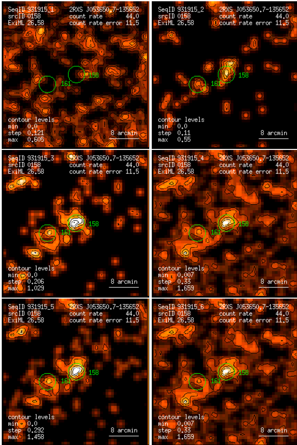
Figure 158: RASS 931915: detection 0158: band rate images, Gaussian filter: (1) PSPC channels 11 – 41, (2) 52 – 90, (3) 91 – 201, (4) 11 – 235, (5) 52 – 201, (6) 11 – 201. Broad band rates in counts/ks. Band rate contour levels in counts/ks/arcmin 2 .
