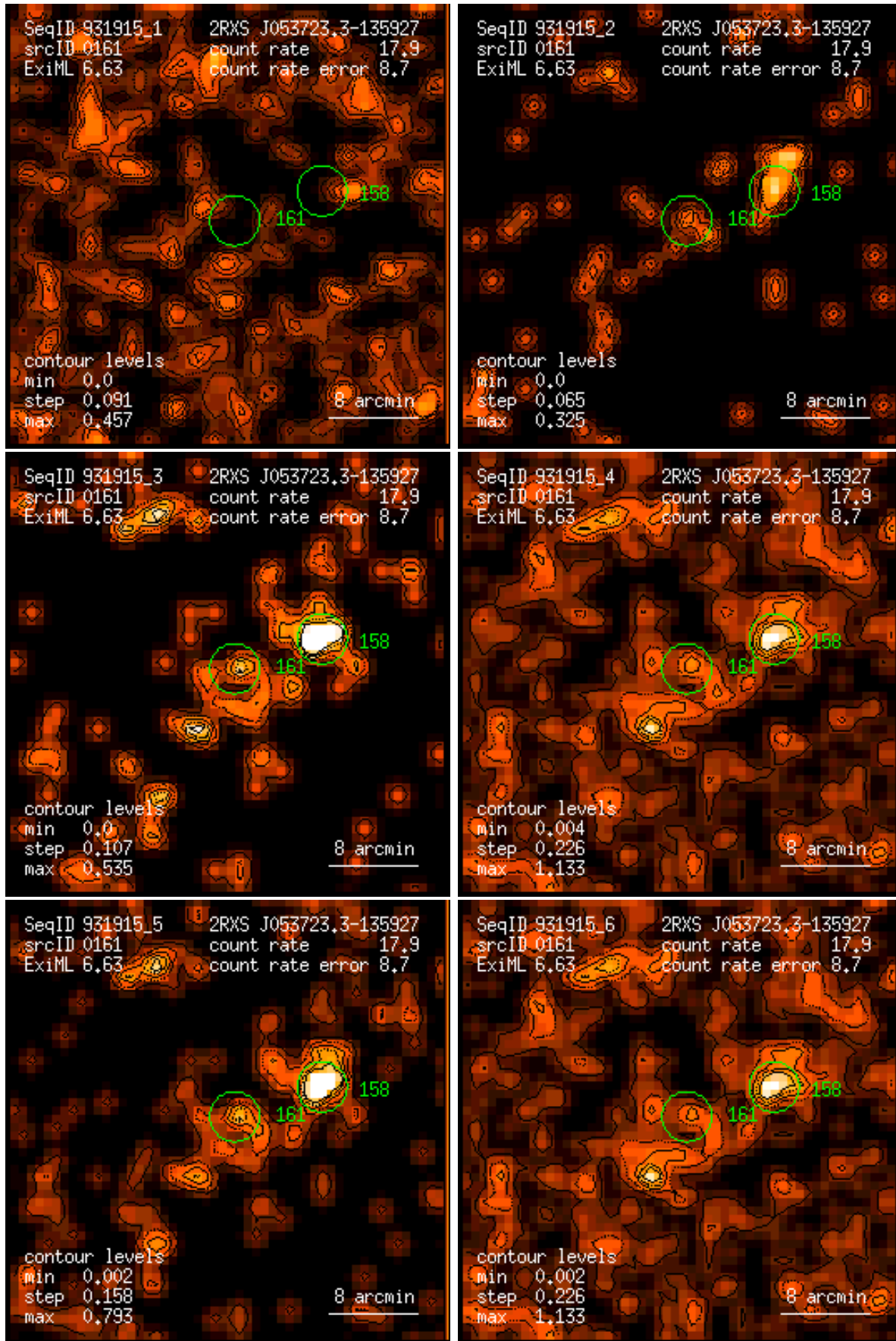
Figure 161: RASS 931915: detection 0161: band rate images, Gaussian filter: (1) PSPC channels 11 – 41, (2) 52 – 90, (3) 91 – 201, (4) 11 – 235, (5) 52 – 201, (6) 11 – 201. Broad band rates in counts/ks. Band rate contour levels in counts/ks/arcmin 2 .
