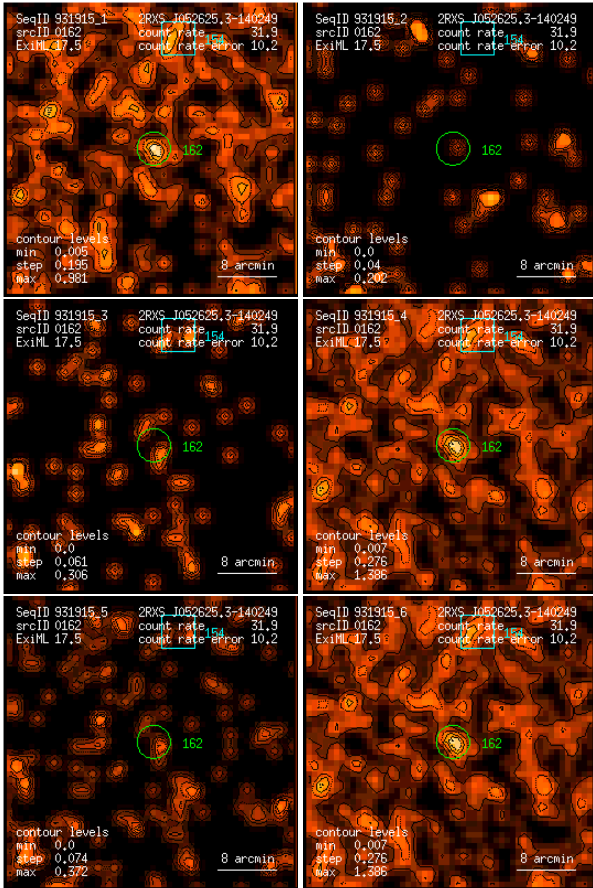
Figure 162: RASS 931915: detection 0162: band rate images, Gaussian filter: (1) PSPC channels 11 – 41, (2) 52 – 90, (3) 91 – 201, (4) 11 – 235, (5) 52 – 201, (6) 11 – 201. Broad band rates in counts/ks. Band rate contour levels in counts/ks/arcmin 2 .
