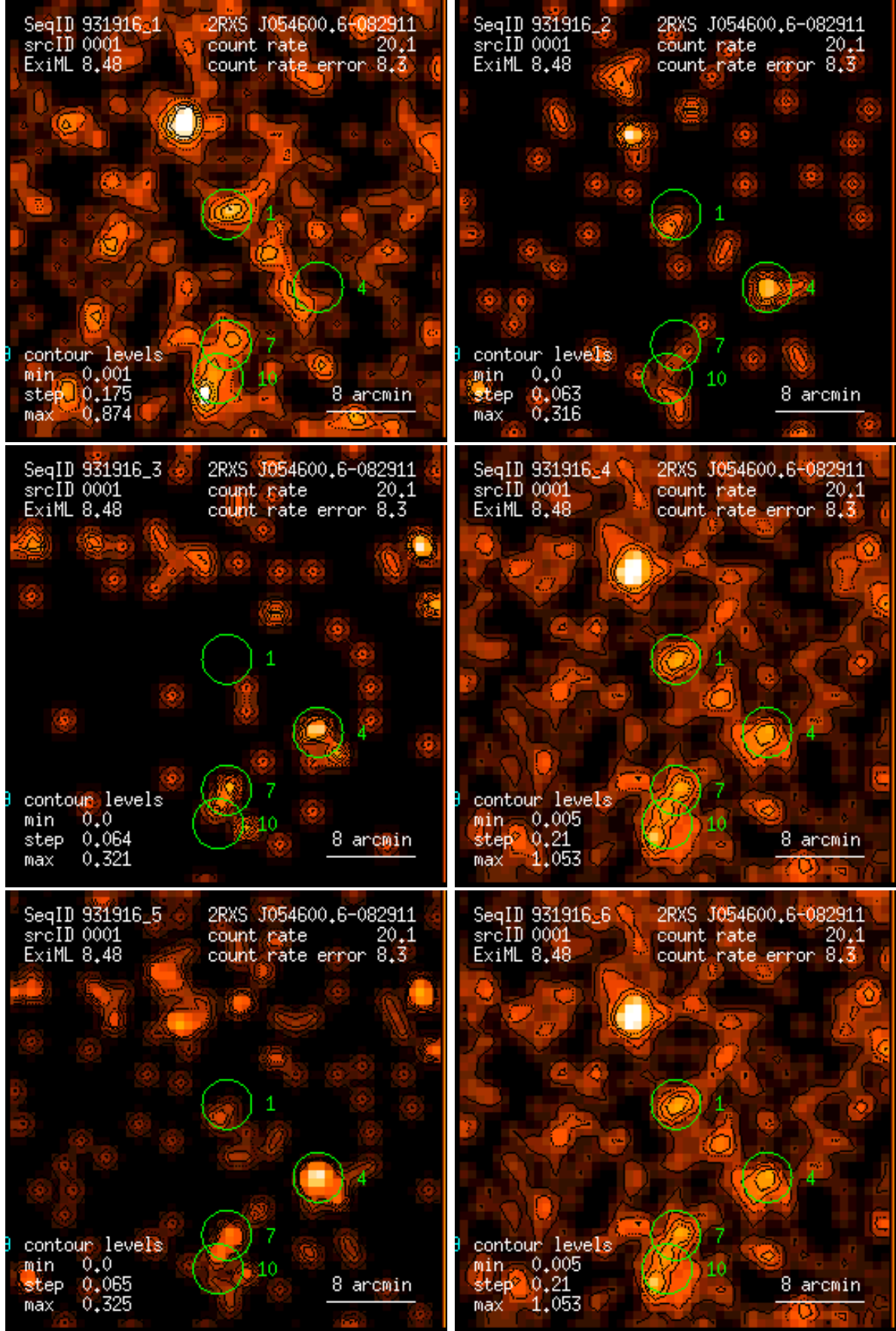
Figure 1: RASS 931916: detection 0001: band rate images, Gaussian filter: (1) PSPC channels 11 – 41, (2) 52 – 90, (3) 91 – 201, (4) 11 – 235, (5) 52 – 201, (6) 11 – 201. Broad band rates in counts/ks. Band rate contour levels in counts/ks/arcmin 2 .
