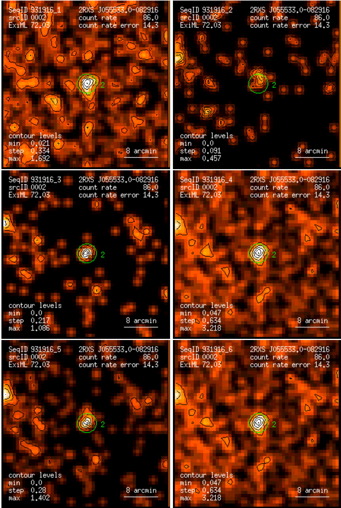
Figure 2: RASS 931916: detection 0002: band rate images, Gaussian filter: (1) PSPC channels 11 – 41, (2) 52 – 90, (3) 91 – 201, (4) 11 – 235, (5) 52 – 201, (6) 11 – 201. Broad band rates in counts/ks. Band rate contour levels in counts/ks/arcmin 2 .
