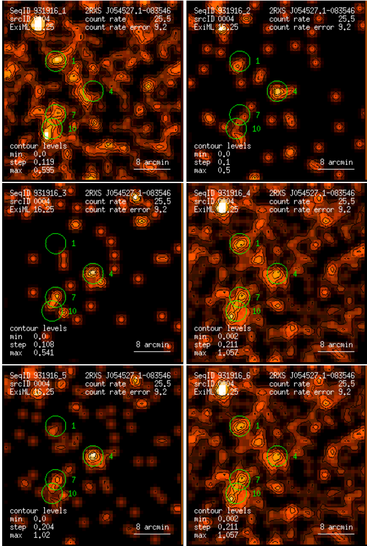
Figure 4: RASS 931916: detection 0004: band rate images, Gaussian filter: (1) PSPC channels 11 – 41, (2) 52 – 90, (3) 91 – 201, (4) 11 – 235, (5) 52 – 201, (6) 11 – 201. Broad band rates in counts/ks. Band rate contour levels in counts/ks/arcmin 2 .
