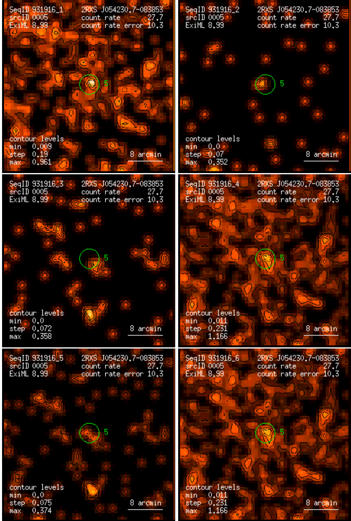
Figure 5: RASS 931916: detection 0005: band rate images, Gaussian filter: (1) PSPC channels 11 – 41, (2) 52 – 90, (3) 91 – 201, (4) 11 – 235, (5) 52 – 201, (6) 11 – 201. Broad band rates in counts/ks. Band rate contour levels in counts/ks/arcmin 2 .
