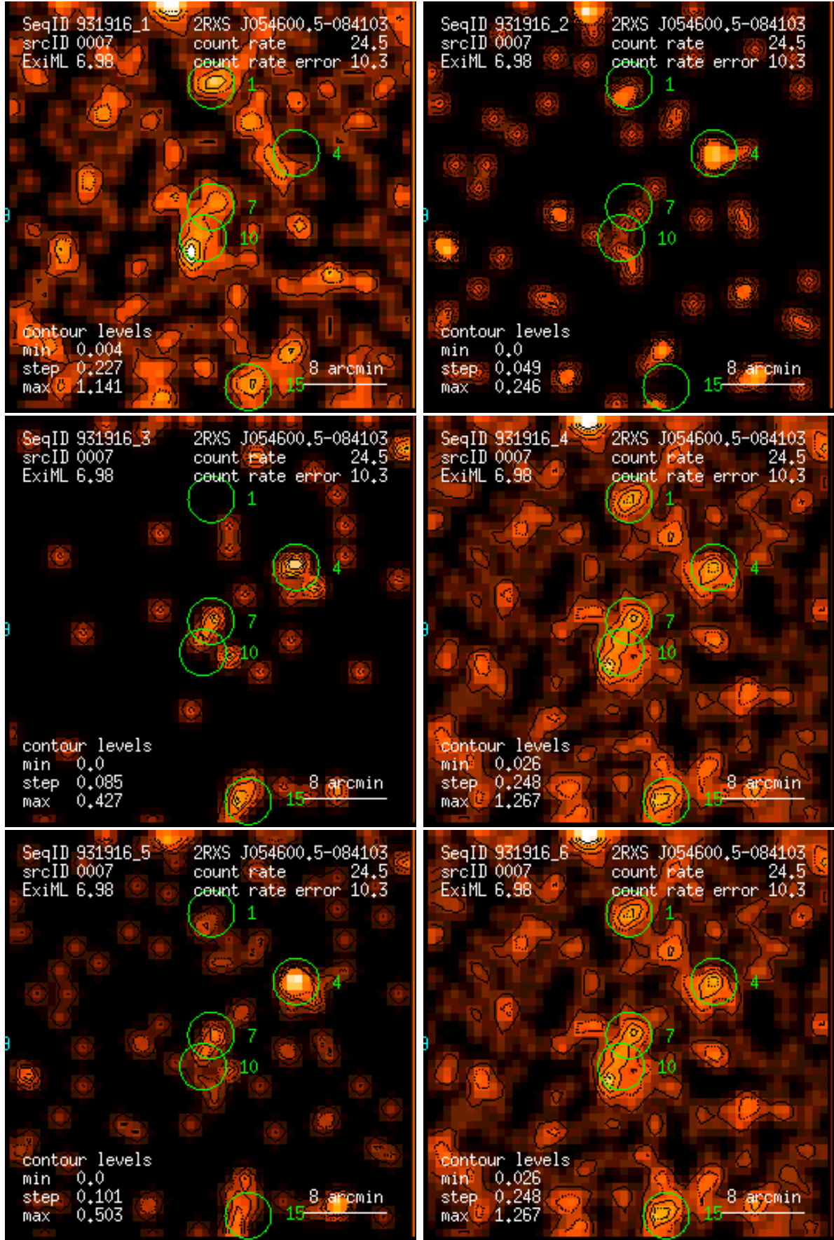
Figure 7: RASS 931916: detection 0007: band rate images, Gaussian filter: (1) PSPC channels 11 – 41, (2) 52 – 90, (3) 91 – 201, (4) 11 – 235, (5) 52 – 201, (6) 11 – 201. Broad band rates in counts/ks. Band rate contour levels in counts/ks/arcmin 2 .
