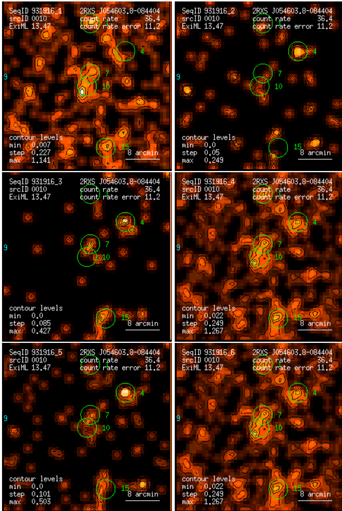
Figure 10: RASS 931916: detection 0010: band rate images, Gaussian filter: (1) PSPC channels 11 – 41, (2) 52 – 90, (3) 91 – 201, (4) 11 – 235, (5) 52 – 201, (6) 11 – 201. Broad band rates in counts/ks. Band rate contour levels in counts/ks/arcmin 2 .
