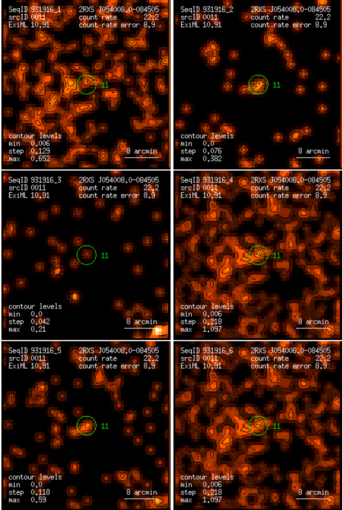
Figure 11: RASS 931916: detection 0011: band rate images, Gaussian filter: (1) PSPC channels 11 – 41, (2) 52 – 90, (3) 91 – 201, (4) 11 – 235, (5) 52 – 201, (6) 11 – 201. Broad band rates in counts/ks. Band rate contour levels in counts/ks/arcmin 2 .
