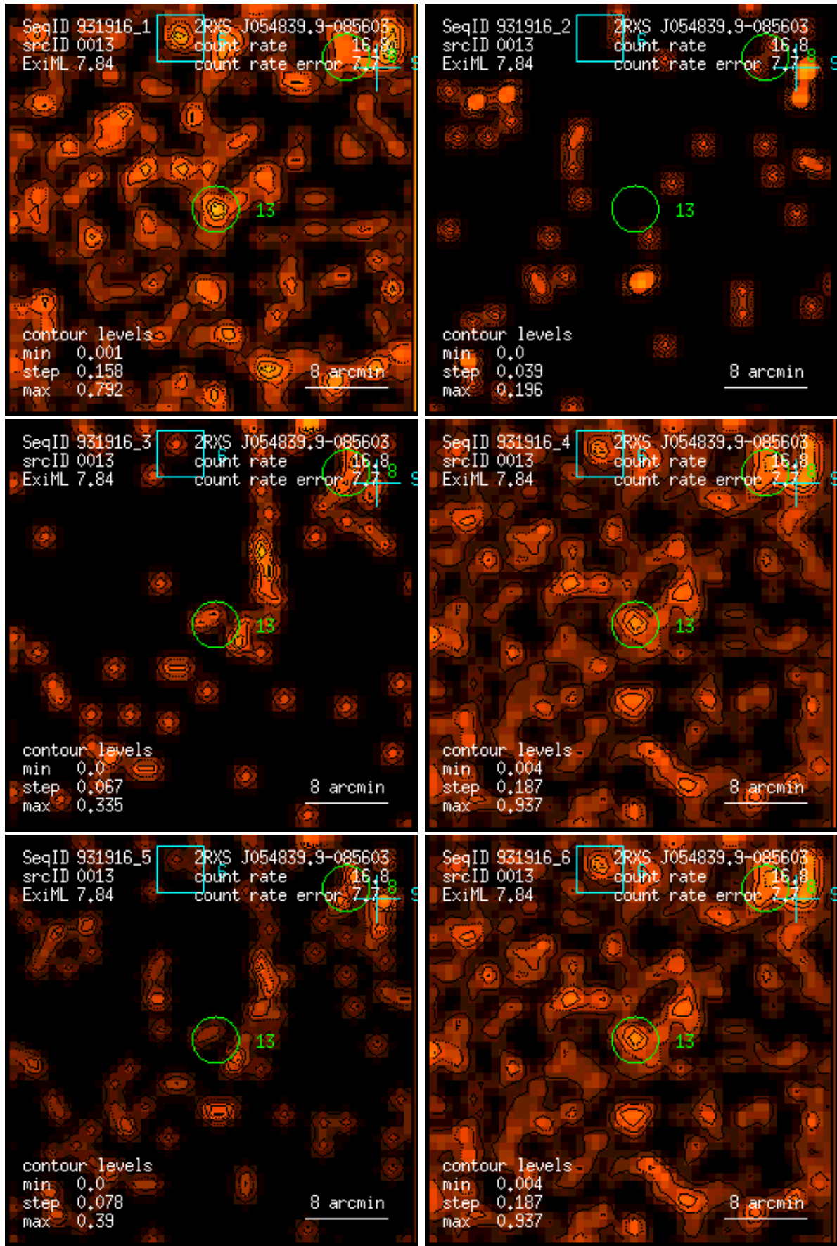
Figure 13: RASS 931916: detection 0013: band rate images, Gaussian filter: (1) PSPC channels 11 – 41, (2) 52 – 90, (3) 91 – 201, (4) 11 – 235, (5) 52 – 201, (6) 11 – 201. Broad band rates in counts/ks. Band rate contour levels in counts/ks/arcmin 2 .
