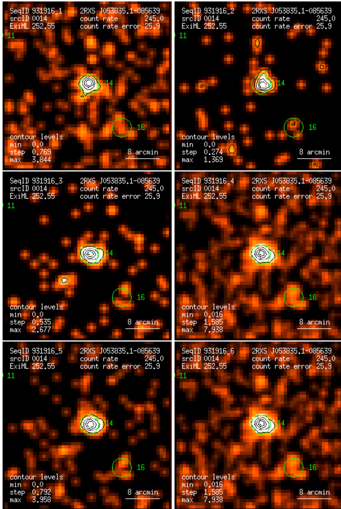
Figure 14: RASS 931916: detection 0014: band rate images, Gaussian filter: (1) PSPC channels 11 – 41, (2) 52 – 90, (3) 91 – 201, (4) 11 – 235, (5) 52 – 201, (6) 11 – 201. Broad band rates in counts/ks. Band rate contour levels in counts/ks/arcmin 2 .
