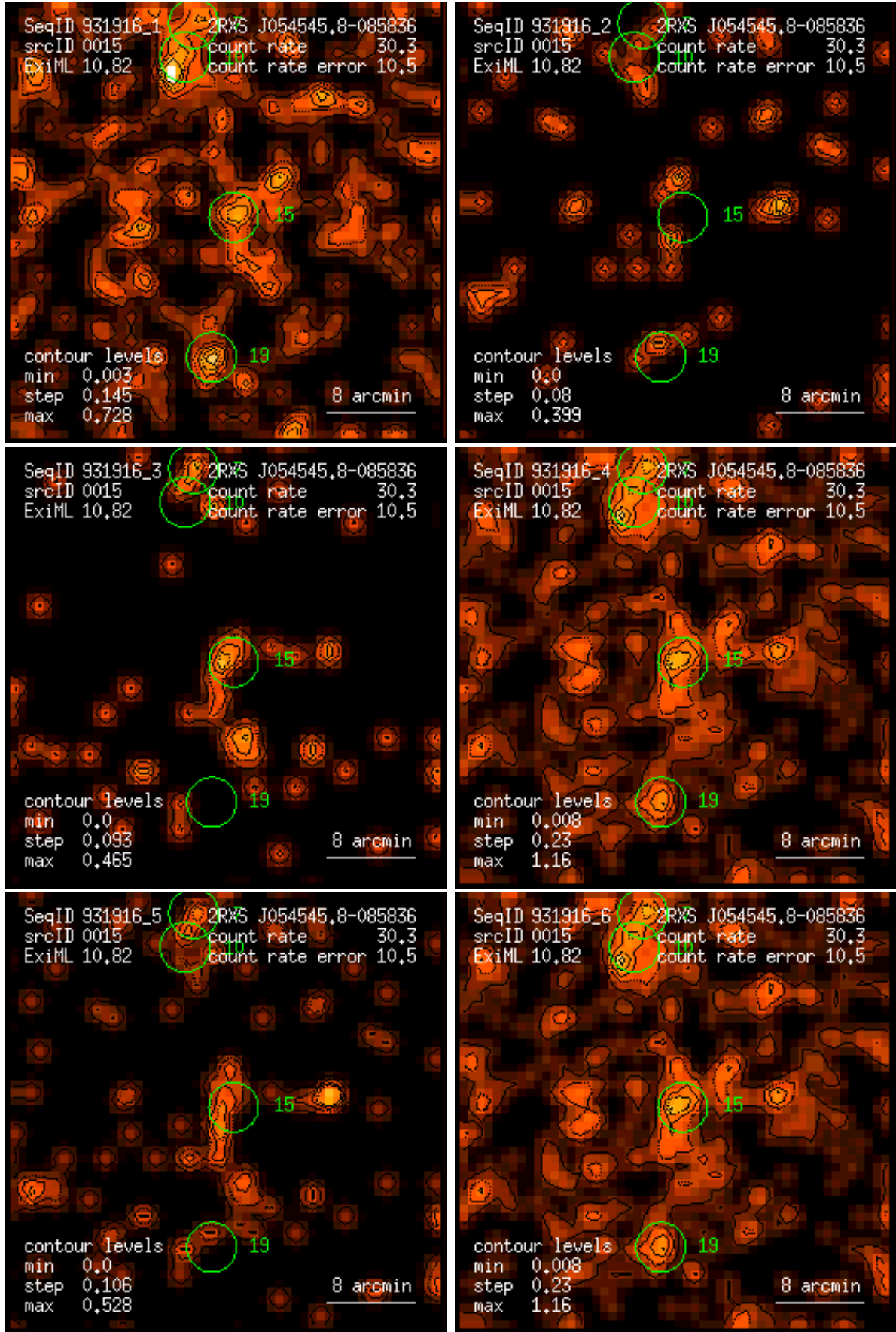
Figure 15: RASS 931916: detection 0015: band rate images, Gaussian filter: (1) PSPC channels 11 – 41, (2) 52 – 90, (3) 91 – 201, (4) 11 – 235, (5) 52 – 201, (6) 11 – 201. Broad band rates in counts/ks. Band rate contour levels in counts/ks/arcmin 2 .
