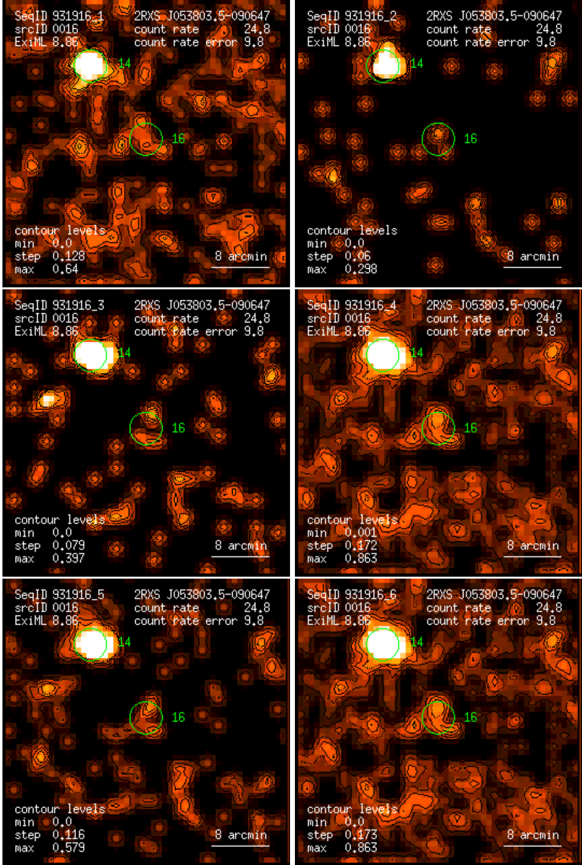
Figure 16: RASS 931916: detection 0016: band rate images, Gaussian filter: (1) PSPC channels 11 – 41, (2) 52 – 90, (3) 91 – 201, (4) 11 – 235, (5) 52 – 201, (6) 11 – 201. Broad band rates in counts/ks. Band rate contour levels in counts/ks/arcmin 2 .
