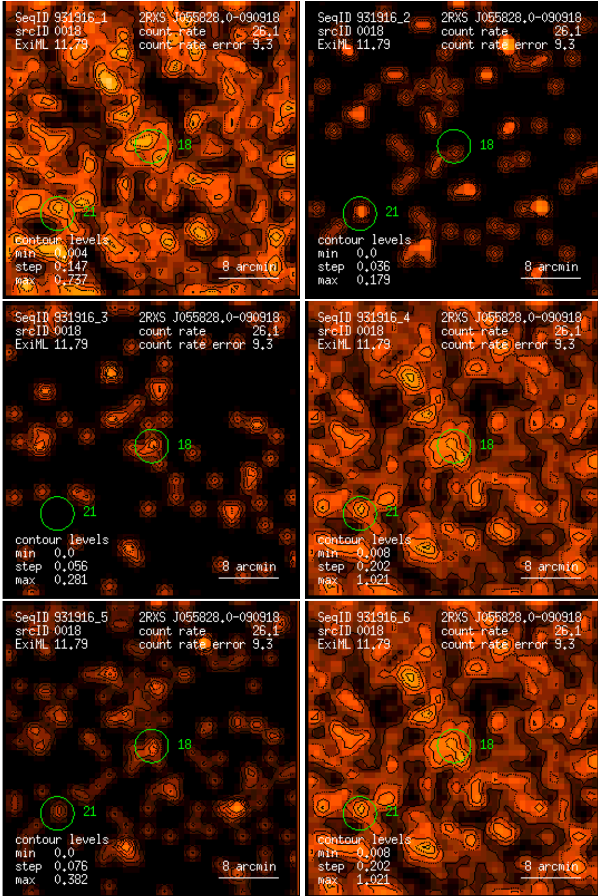
Figure 18: RASS 931916: detection 0018: band rate images, Gaussian filter: (1) PSPC channels 11 – 41, (2) 52 – 90, (3) 91 – 201, (4) 11 – 235, (5) 52 – 201, (6) 11 – 201. Broad band rates in counts/ks. Band rate contour levels in counts/ks/arcmin 2 .
