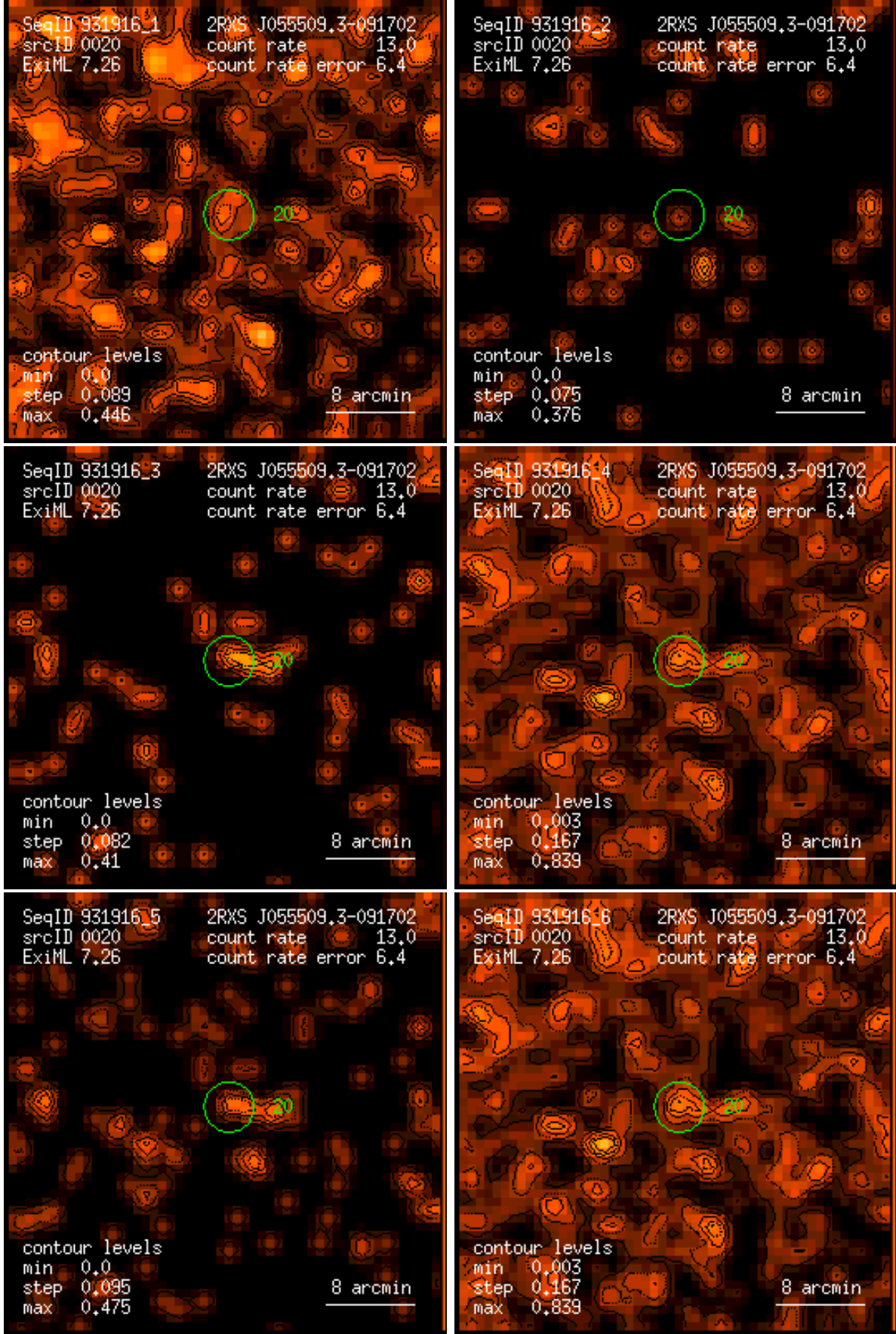
Figure 20: RASS 931916: detection 0020: band rate images, Gaussian filter: (1) PSPC channels 11 – 41, (2) 52 – 90, (3) 91 – 201, (4) 11 – 235, (5) 52 – 201, (6) 11 – 201. Broad band rates in counts/ks. Band rate contour levels in counts/ks/arcmin 2 .
