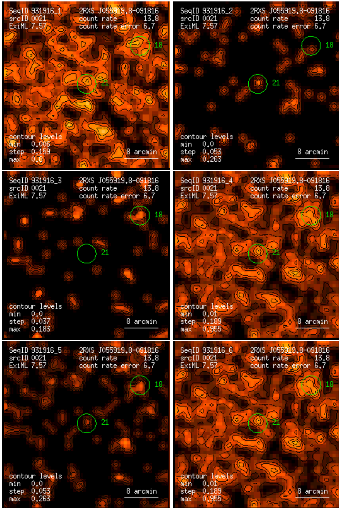
Figure 21: RASS 931916: detection 0021: band rate images, Gaussian filter: (1) PSPC channels 11 – 41, (2) 52 – 90, (3) 91 – 201, (4) 11 – 235, (5) 52 – 201, (6) 11 – 201. Broad band rates in counts/ks. Band rate contour levels in counts/ks/arcmin 2 .
