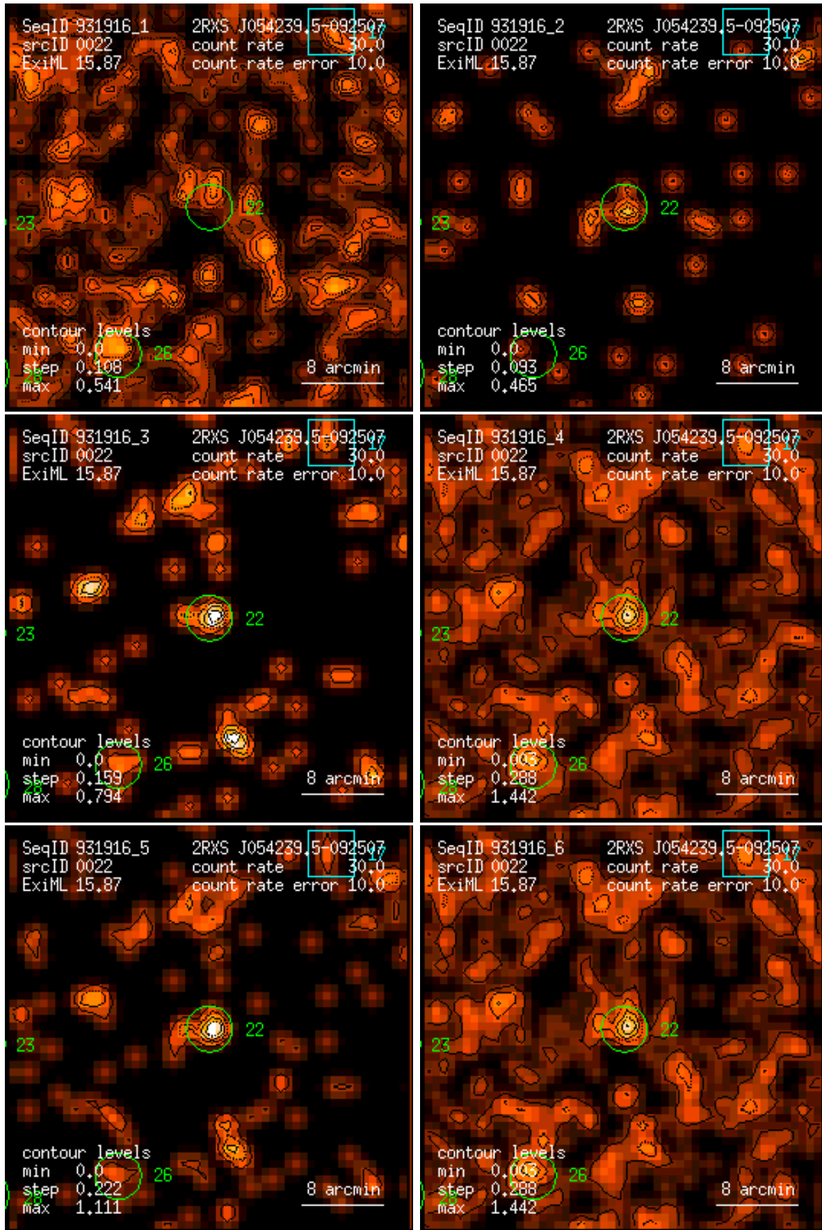
Figure 22: RASS 931916: detection 0022: band rate images, Gaussian filter: (1) PSPC channels 11 – 41, (2) 52 – 90, (3) 91 – 201, (4) 11 – 235, (5) 52 – 201, (6) 11 – 201. Broad band rates in counts/ks. Band rate contour levels in counts/ks/arcmin 2 .
