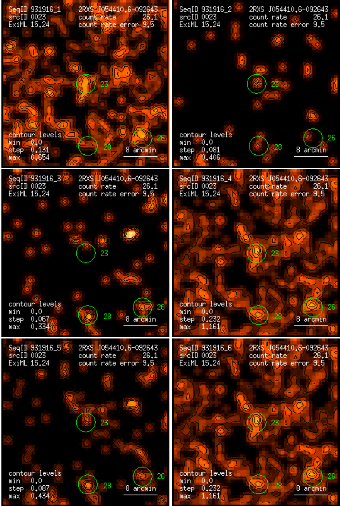
Figure 23: RASS 931916: detection 0023: band rate images, Gaussian filter: (1) PSPC channels 11 – 41, (2) 52 – 90, (3) 91 – 201, (4) 11 – 235, (5) 52 – 201, (6) 11 – 201. Broad band rates in counts/ks. Band rate contour levels in counts/ks/arcmin 2 .
