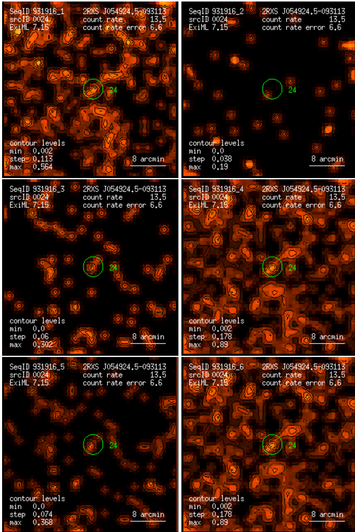
Figure 24: RASS 931916: detection 0024: band rate images, Gaussian filter: (1) PSPC channels 11 – 41, (2) 52 – 90, (3) 91 – 201, (4) 11 – 235, (5) 52 – 201, (6) 11 – 201. Broad band rates in counts/ks. Band rate contour levels in counts/ks/arcmin 2 .
