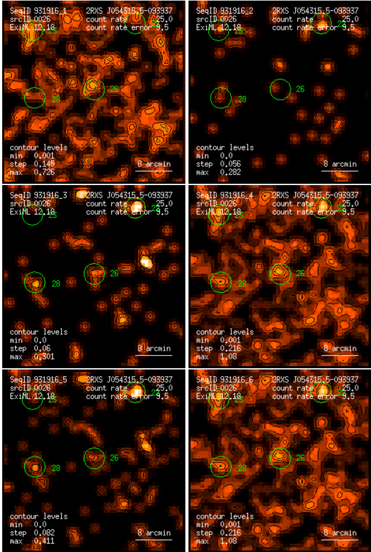
Figure 26: RASS 931916: detection 0026: band rate images, Gaussian filter: (1) PSPC channels 11 – 41, (2) 52 – 90, (3) 91 – 201, (4) 11 – 235, (5) 52 – 201, (6) 11 – 201. Broad band rates in counts/ks. Band rate contour levels in counts/ks/arcmin 2 .
