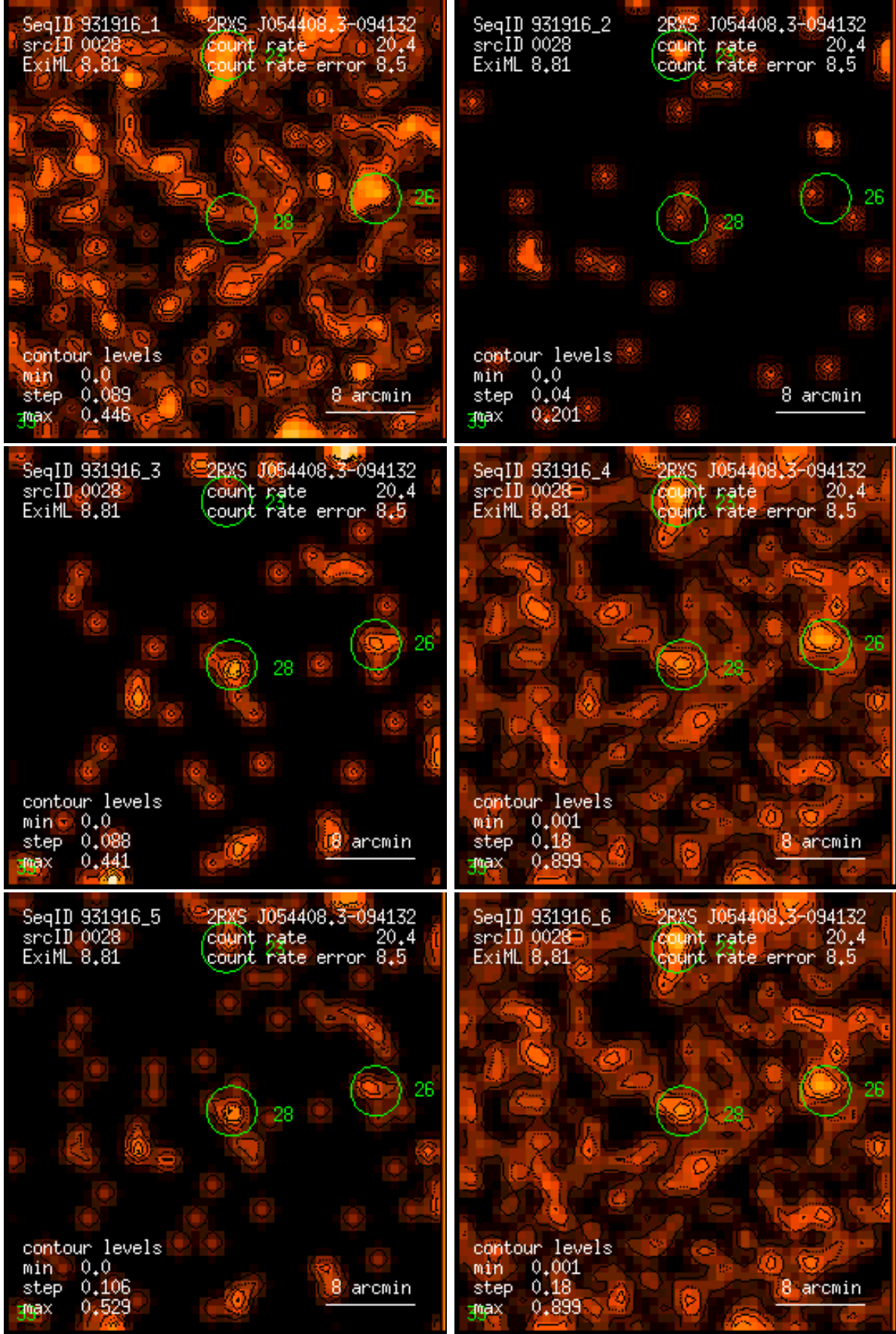
Figure 28: RASS 931916: detection 0028: band rate images, Gaussian filter: (1) PSPC channels 11 – 41, (2) 52 – 90, (3) 91 – 201, (4) 11 – 235, (5) 52 – 201, (6) 11 – 201. Broad band rates in counts/ks. Band rate contour levels in counts/ks/arcmin 2 .
