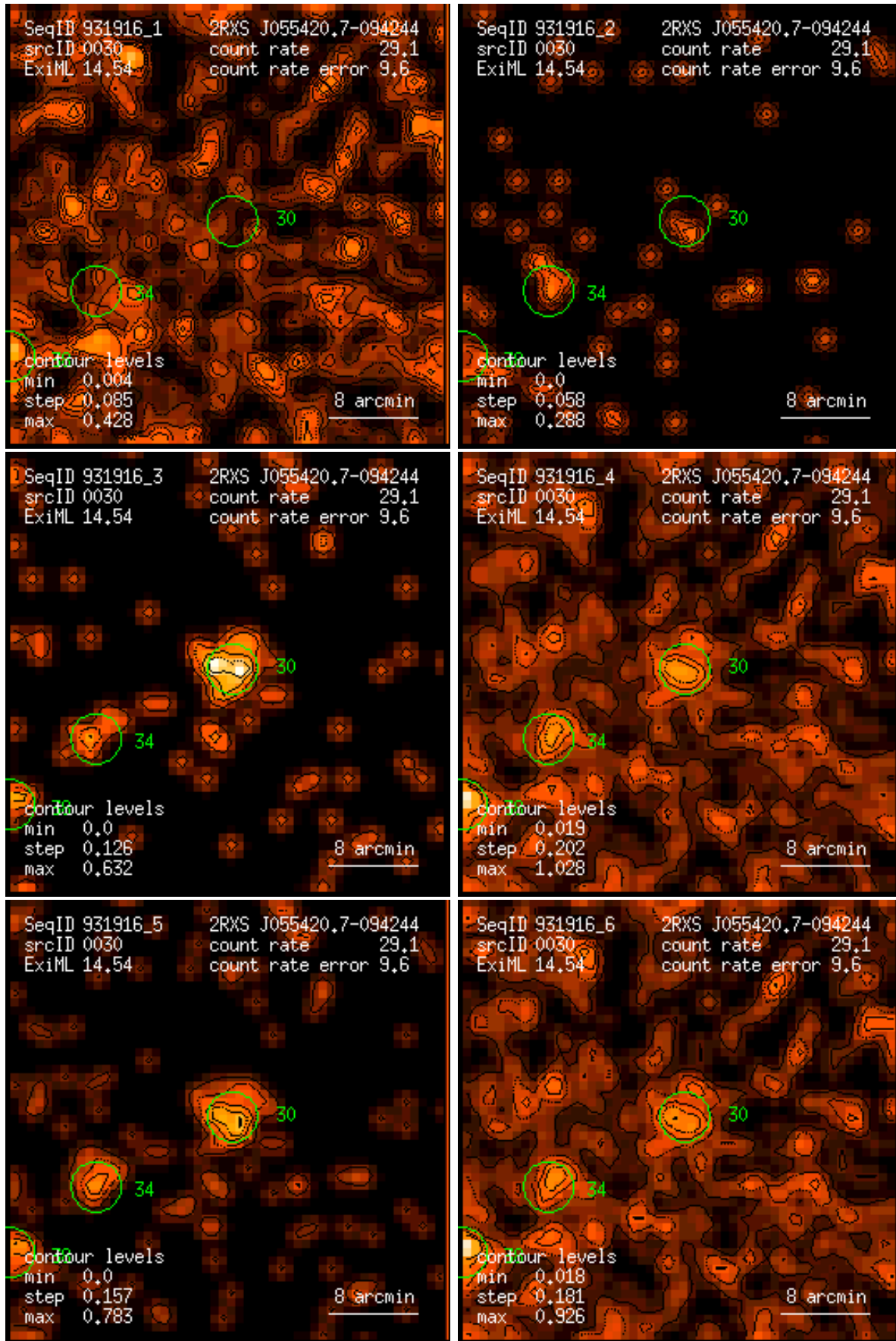
Figure 30: RASS 931916: detection 0030: band rate images, Gaussian filter: (1) PSPC channels 11 – 41, (2) 52 – 90, (3) 91 – 201, (4) 11 – 235, (5) 52 – 201, (6) 11 – 201. Broad band rates in counts/ks. Band rate contour levels in counts/ks/arcmin 2 .
